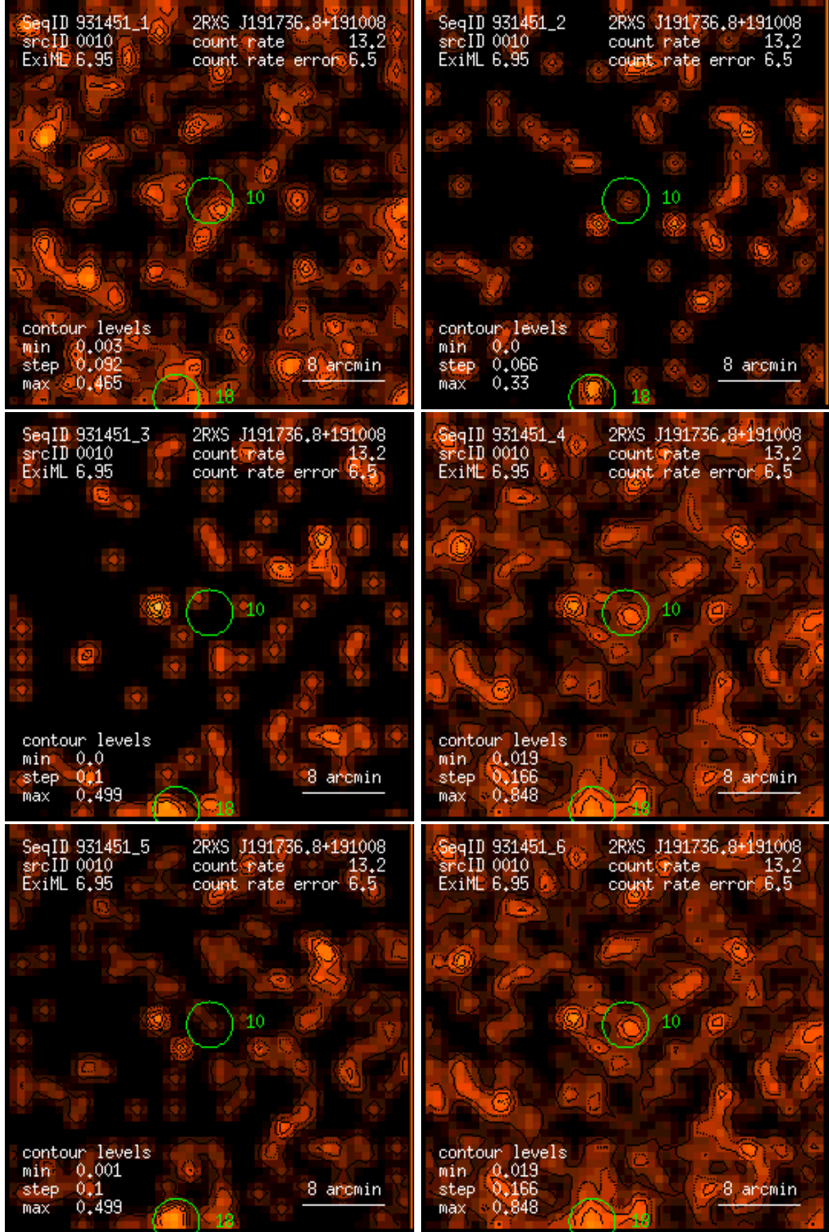
Figure 10: RASS 931451: detection 0010: band rate images, Gaussian filter: (1) PSPC channels 11 – 41, (2) 52 – 90, (3) 91 – 201, (4) 11 – 235, (5) 52 – 201, (6) 11 – 201. Broad band rates in counts/ks. Band rate contour levels in counts/ks/arcmin 2 .
