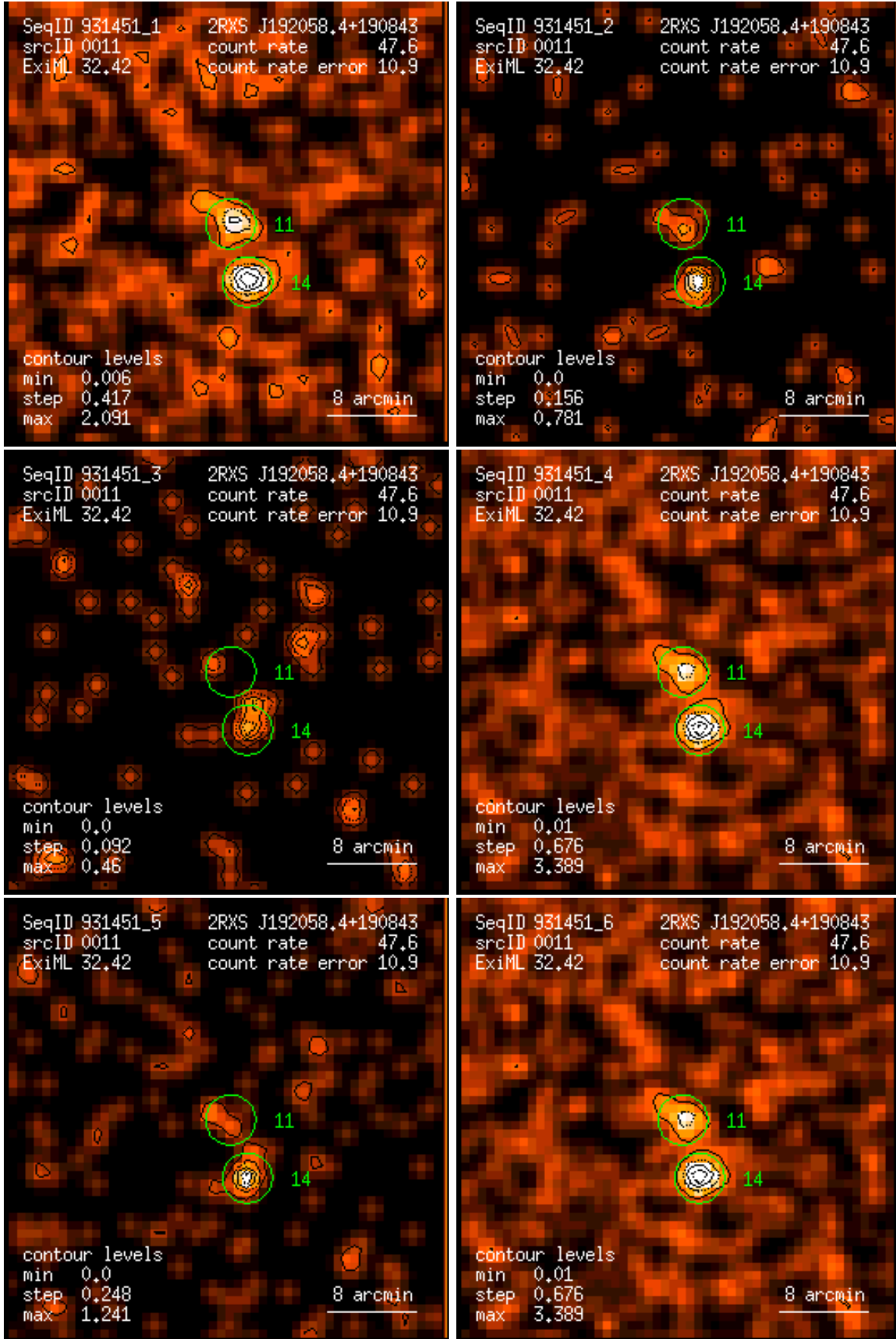
Figure 11: RASS 931451: detection 0011: band rate images, Gaussian filter: (1) PSPC channels 11 – 41, (2) 52 – 90, (3) 91 – 201, (4) 11 – 235, (5) 52 – 201, (6) 11 – 201. Broad band rates in counts/ks. Band rate contour levels in counts/ks/arcmin 2 .
