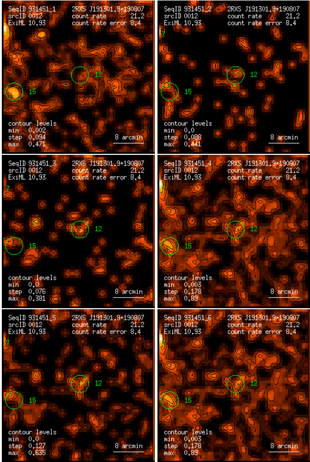
Figure 12: RASS 931451: detection 0012: band rate images, Gaussian filter: (1) PSPC channels 11 – 41, (2) 52 – 90, (3) 91 – 201, (4) 11 – 235, (5) 52 – 201, (6) 11 – 201. Broad band rates in counts/ks. Band rate contour levels in counts/ks/arcmin 2 .
