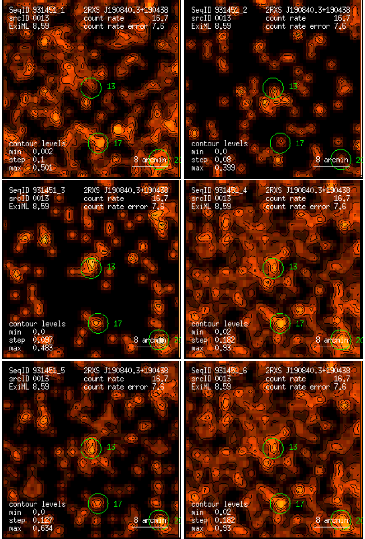
Figure 13: RASS 931451: detection 0013: band rate images, Gaussian filter: (1) PSPC channels 11 – 41, (2) 52 – 90, (3) 91 – 201, (4) 11 – 235, (5) 52 – 201, (6) 11 – 201. Broad band rates in counts/ks. Band rate contour levels in counts/ks/arcmin 2 .
