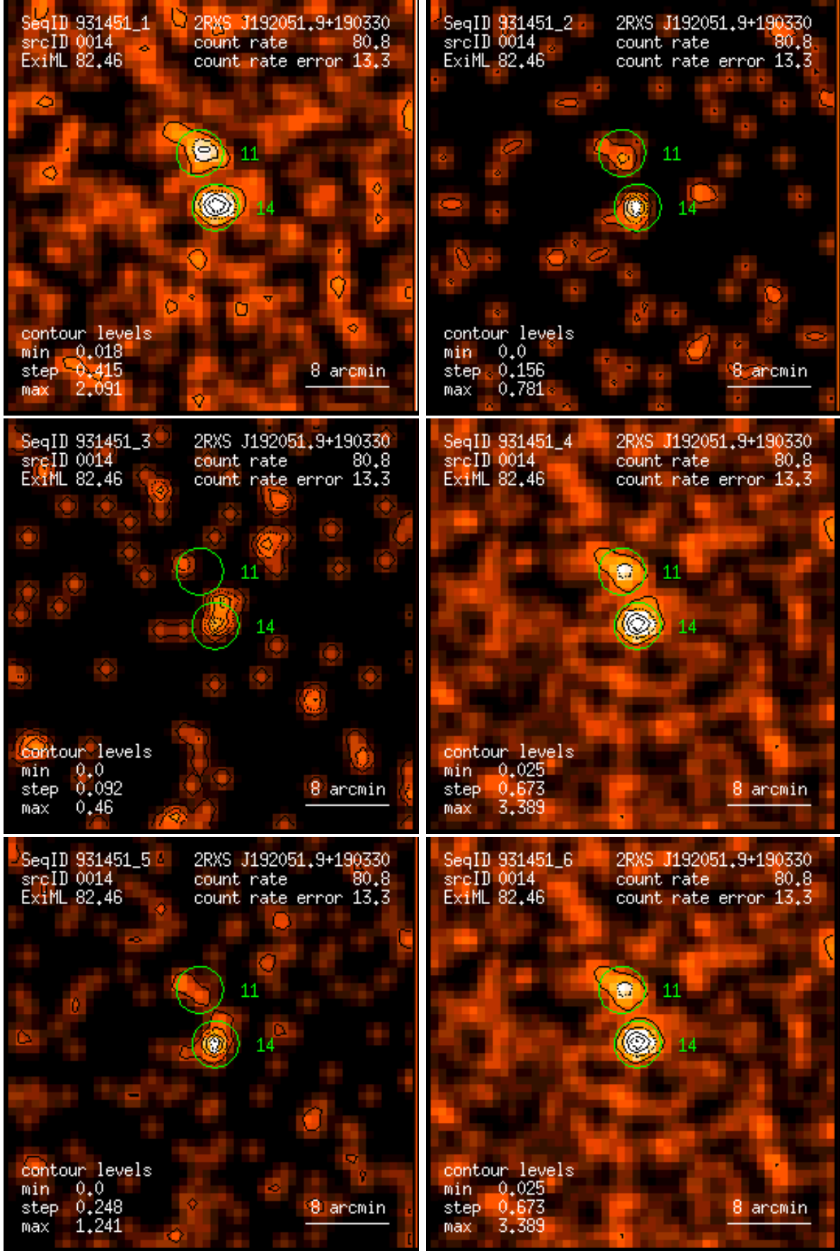
Figure 14: RASS 931451: detection 0014: band rate images, Gaussian filter: (1) PSPC channels 11 – 41, (2) 52 – 90, (3) 91 – 201, (4) 11 – 235, (5) 52 – 201, (6) 11 – 201. Broad band rates in counts/ks. Band rate contour levels in counts/ks/arcmin 2 .
