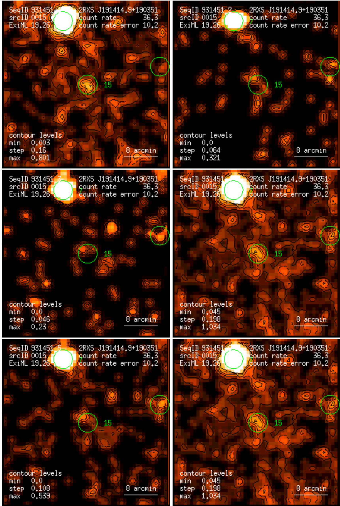
Figure 15: RASS 931451: detection 0015: band rate images, Gaussian filter: (1) PSPC channels 11 – 41, (2) 52 – 90, (3) 91 – 201, (4) 11 – 235, (5) 52 – 201, (6) 11 – 201. Broad band rates in counts/ks. Band rate contour levels in counts/ks/arcmin 2 .
