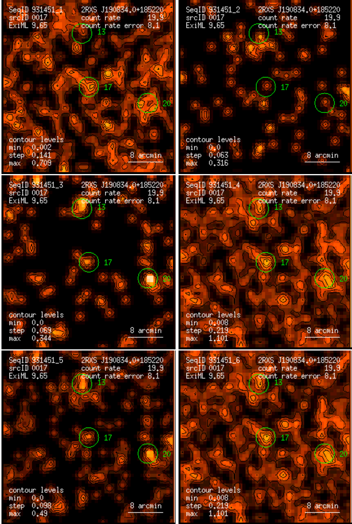
Figure 17: RASS 931451: detection 0017: band rate images, Gaussian filter: (1) PSPC channels 11 – 41, (2) 52 – 90, (3) 91 – 201, (4) 11 – 235, (5) 52 – 201, (6) 11 – 201. Broad band rates in counts/ks. Band rate contour levels in counts/ks/arcmin 2 .
