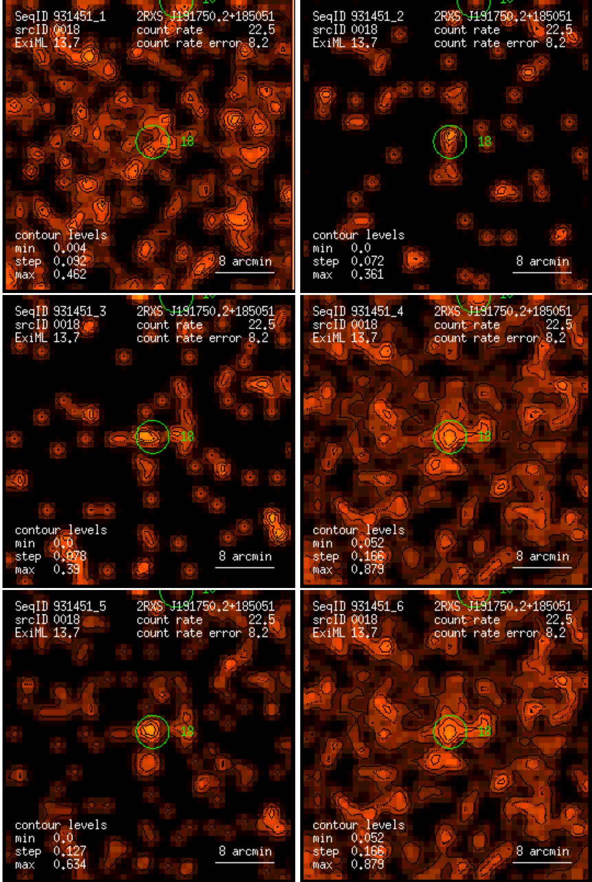
Figure 18: RASS 931451: detection 0018: band rate images, Gaussian filter: (1) PSPC channels 11 – 41, (2) 52 – 90, (3) 91 – 201, (4) 11 – 235, (5) 52 – 201, (6) 11 – 201. Broad band rates in counts/ks. Band rate contour levels in counts/ks/arcmin 2 .
