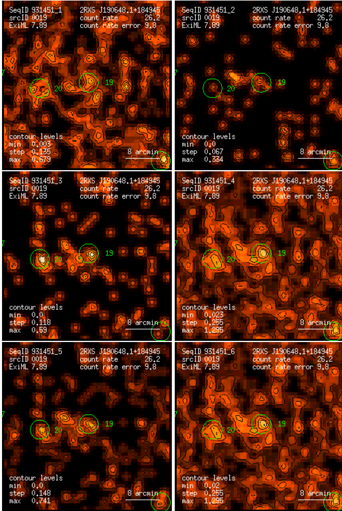
Figure 19: RASS 931451: detection 0019: band rate images, Gaussian filter: (1) PSPC channels 11 – 41, (2) 52 – 90, (3) 91 – 201, (4) 11 – 235, (5) 52 – 201, (6) 11 – 201. Broad band rates in counts/ks. Band rate contour levels in counts/ks/arcmin 2 .
