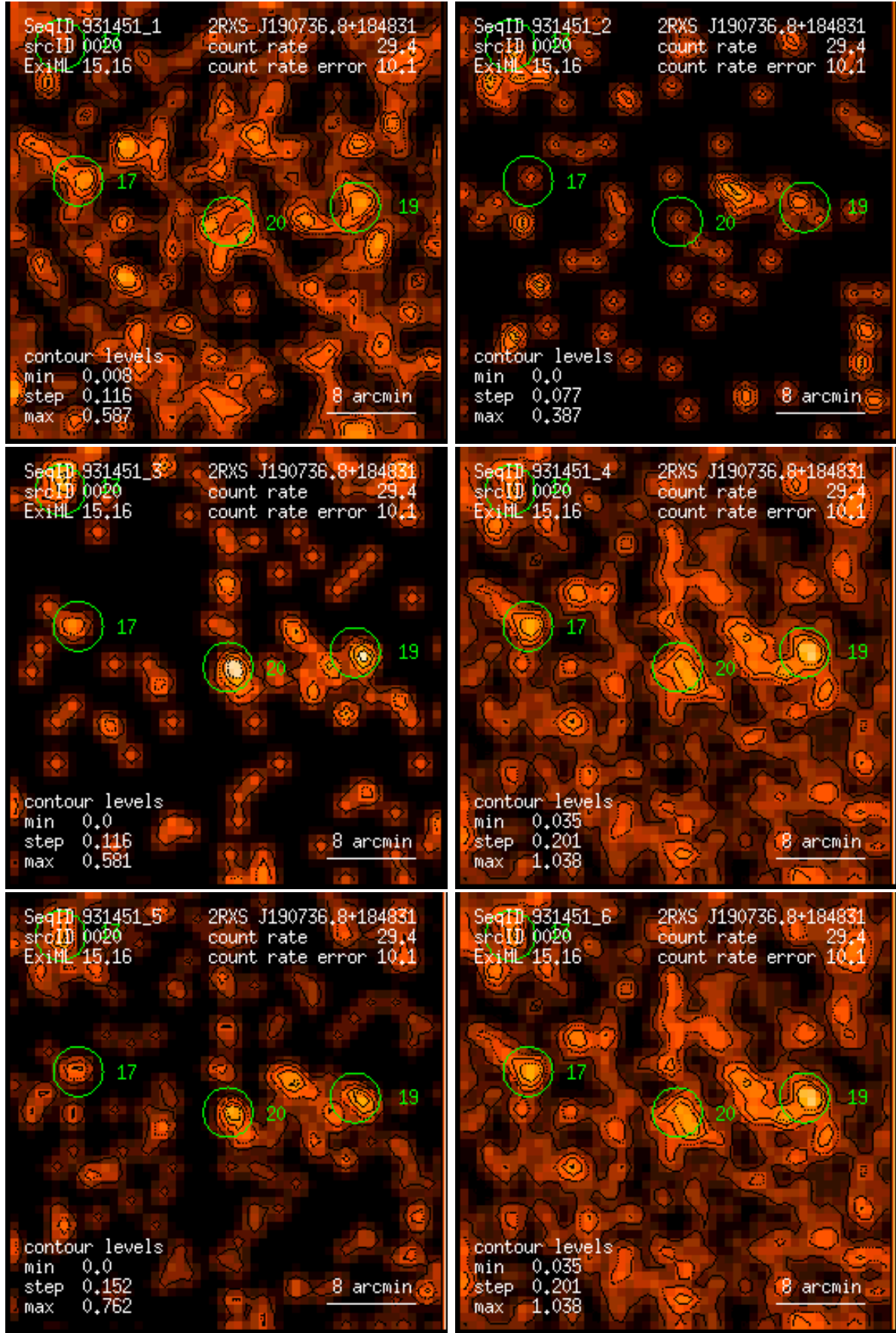
Figure 20: RASS 931451: detection 0020: band rate images, Gaussian filter: (1) PSPC channels 11 – 41, (2) 52 – 90, (3) 91 – 201, (4) 11 – 235, (5) 52 – 201, (6) 11 – 201. Broad band rates in counts/ks. Band rate contour levels in counts/ks/arcmin 2 .
