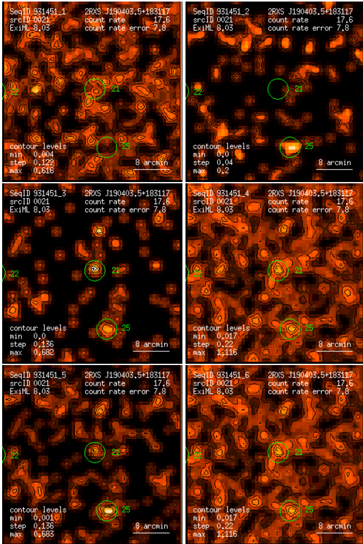
Figure 21: RASS 931451: detection 0021: band rate images, Gaussian filter: (1) PSPC channels 11 – 41, (2) 52 – 90, (3) 91 – 201, (4) 11 – 235, (5) 52 – 201, (6) 11 – 201. Broad band rates in counts/ks. Band rate contour levels in counts/ks/arcmin 2 .
