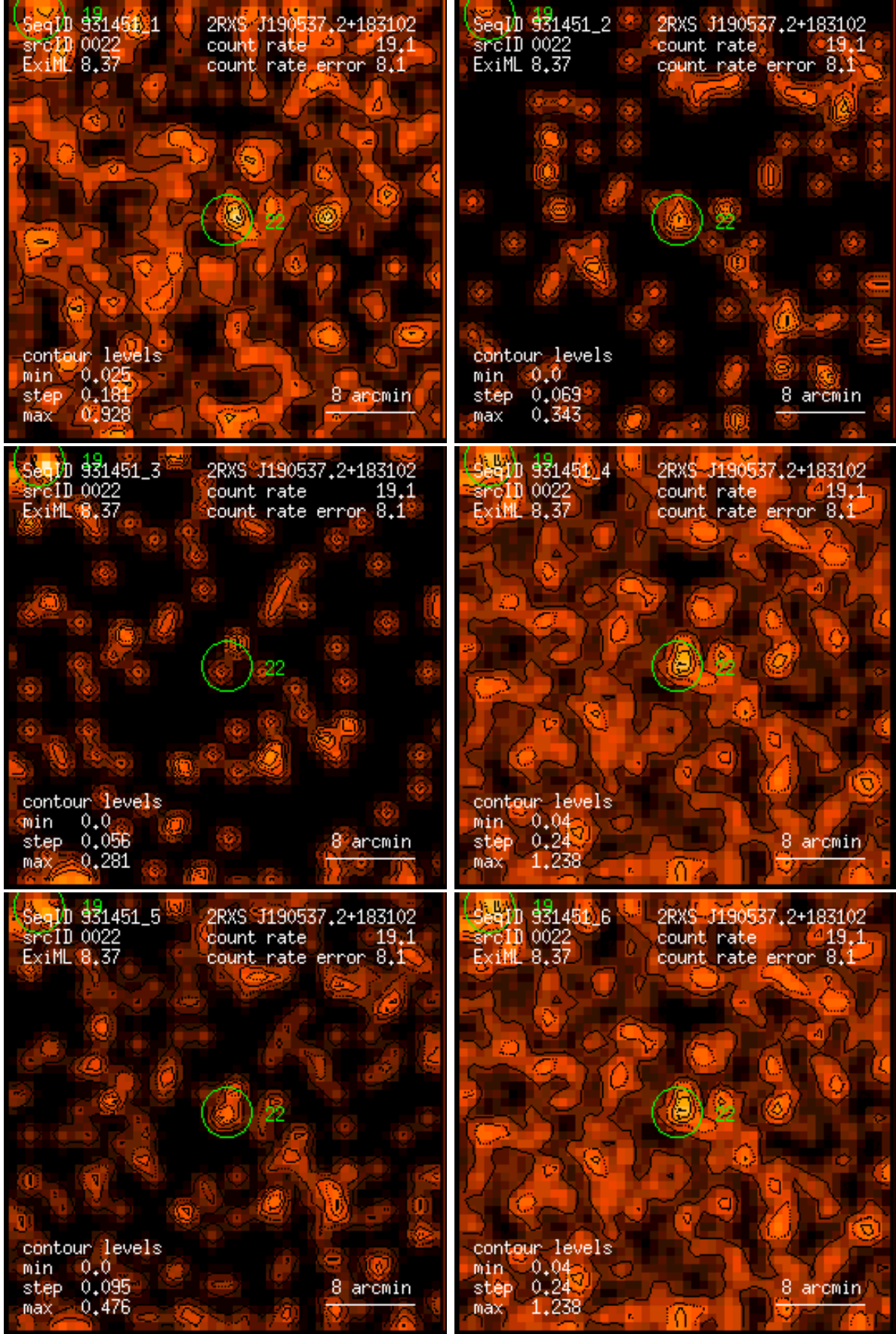
Figure 22: RASS 931451: detection 0022: band rate images, Gaussian filter: (1) PSPC channels 11 – 41, (2) 52 – 90, (3) 91 – 201, (4) 11 – 235, (5) 52 – 201, (6) 11 – 201. Broad band rates in counts/ks. Band rate contour levels in counts/ks/arcmin 2 .
