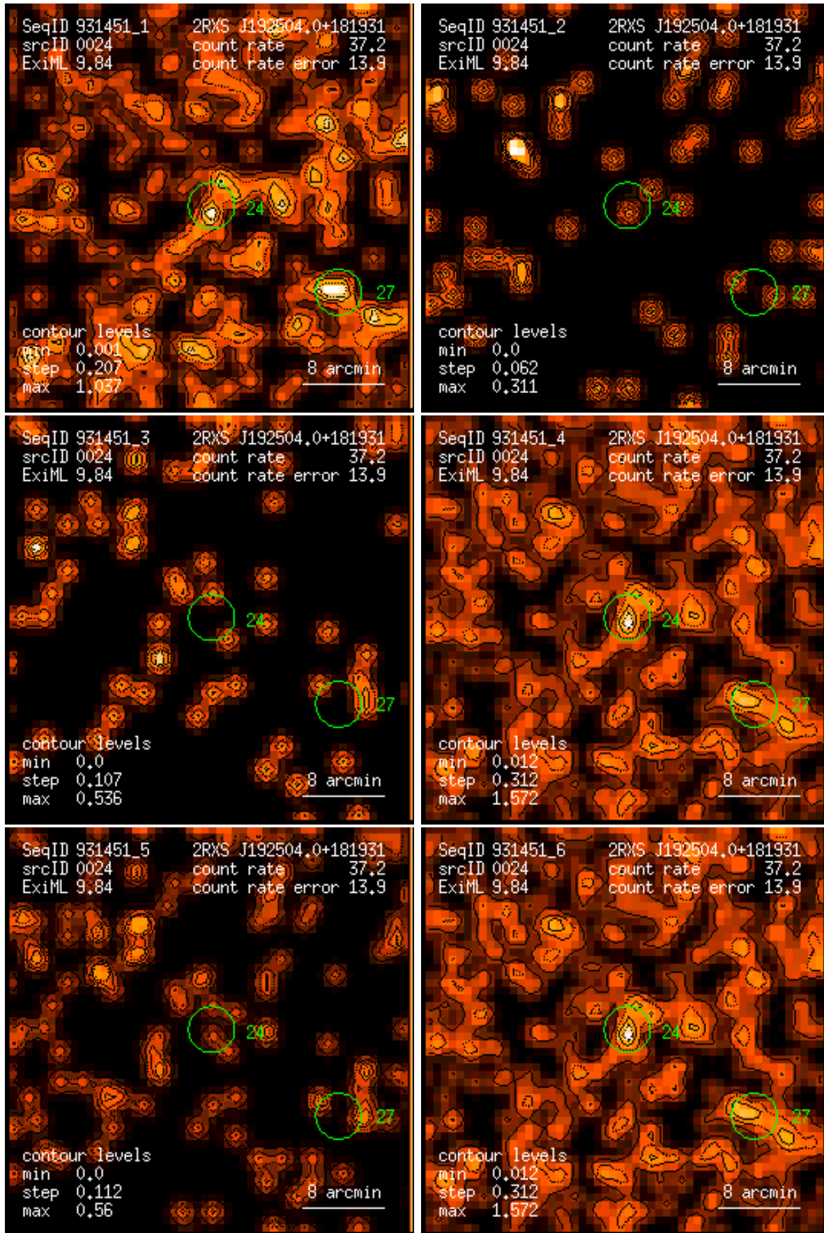
Figure 24: RASS 931451: detection 0024: band rate images, Gaussian filter: (1) PSPC channels 11 – 41, (2) 52 – 90, (3) 91 – 201, (4) 11 – 235, (5) 52 – 201, (6) 11 – 201. Broad band rates in counts/ks. Band rate contour levels in counts/ks/arcmin 2 .
