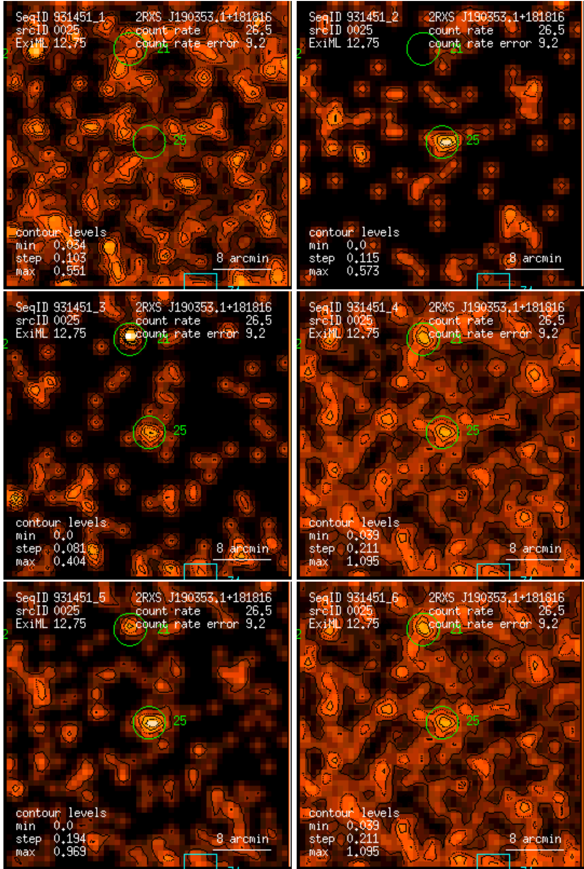
Figure 25: RASS 931451: detection 0025: band rate images, Gaussian filter: (1) PSPC channels 11 – 41, (2) 52 – 90, (3) 91 – 201, (4) 11 – 235, (5) 52 – 201, (6) 11 – 201. Broad band rates in counts/ks. Band rate contour levels in counts/ks/arcmin 2 .
