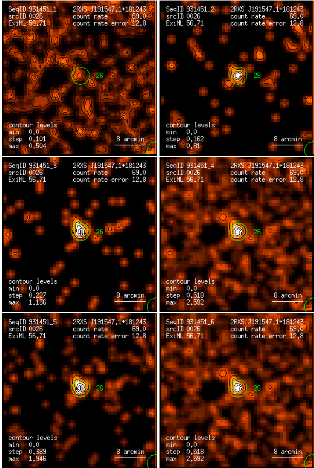
Figure 26: RASS 931451: detection 0026: band rate images, Gaussian filter: (1) PSPC channels 11 – 41, (2) 52 – 90, (3) 91 – 201, (4) 11 – 235, (5) 52 – 201, (6) 11 – 201. Broad band rates in counts/ks. Band rate contour levels in counts/ks/arcmin 2 .
