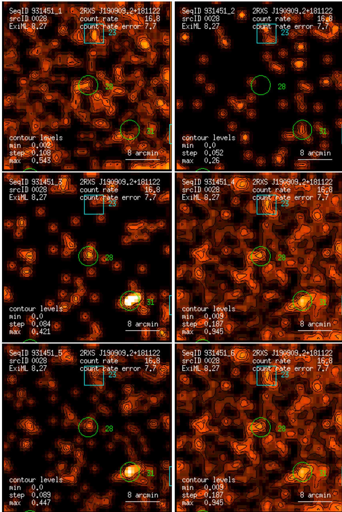
Figure 28: RASS 931451: detection 0028: band rate images, Gaussian filter: (1) PSPC channels 11 – 41, (2) 52 – 90, (3) 91 – 201, (4) 11 – 235, (5) 52 – 201, (6) 11 – 201. Broad band rates in counts/ks. Band rate contour levels in counts/ks/arcmin 2 .
