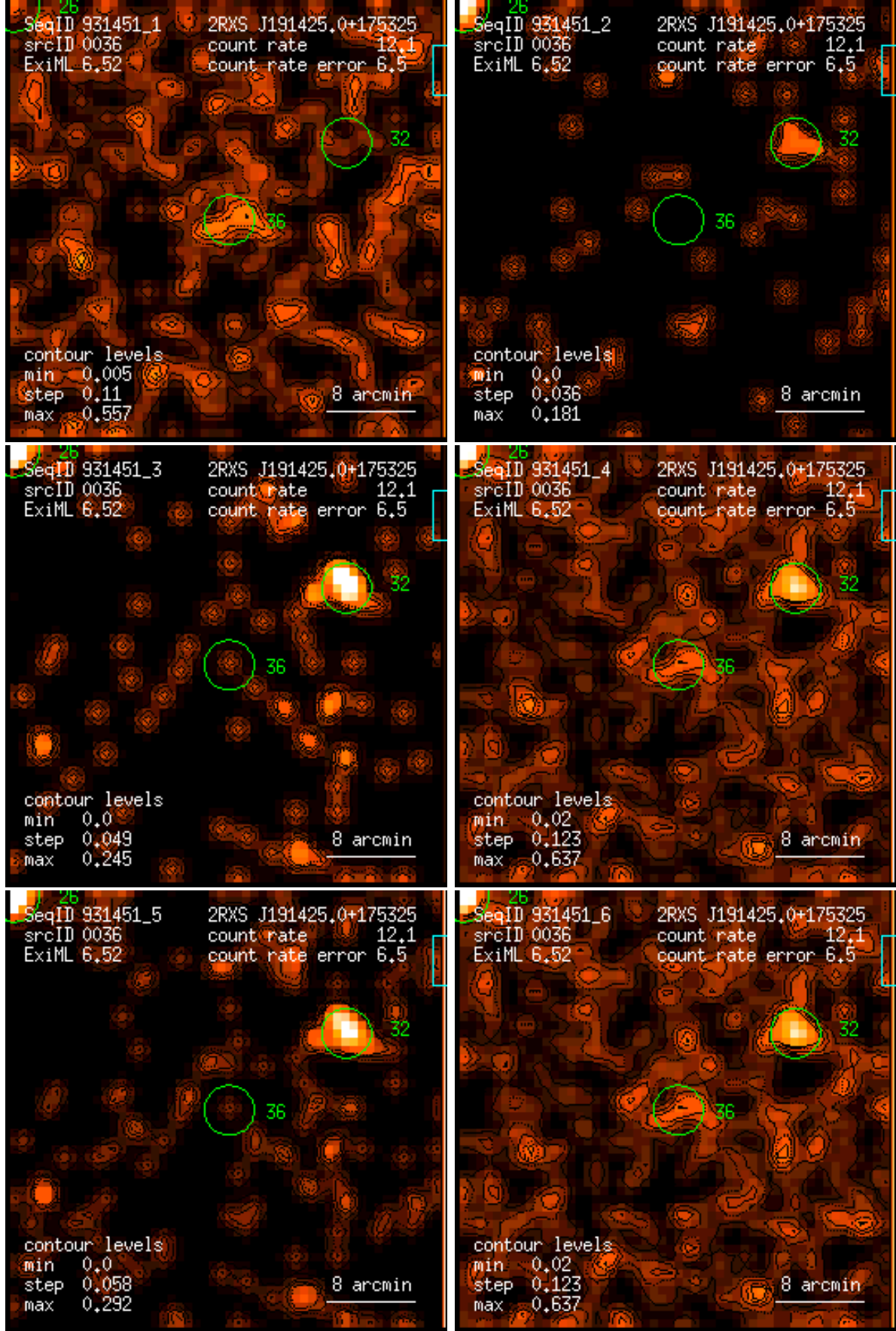
Figure 36: RASS 931451: detection 0036: band rate images, Gaussian filter: (1) PSPC channels 11 – 41, (2) 52 – 90, (3) 91 – 201, (4) 11 – 235, (5) 52 – 201, (6) 11 – 201. Broad band rates in counts/ks. Band rate contour levels in counts/ks/arcmin 2 .
