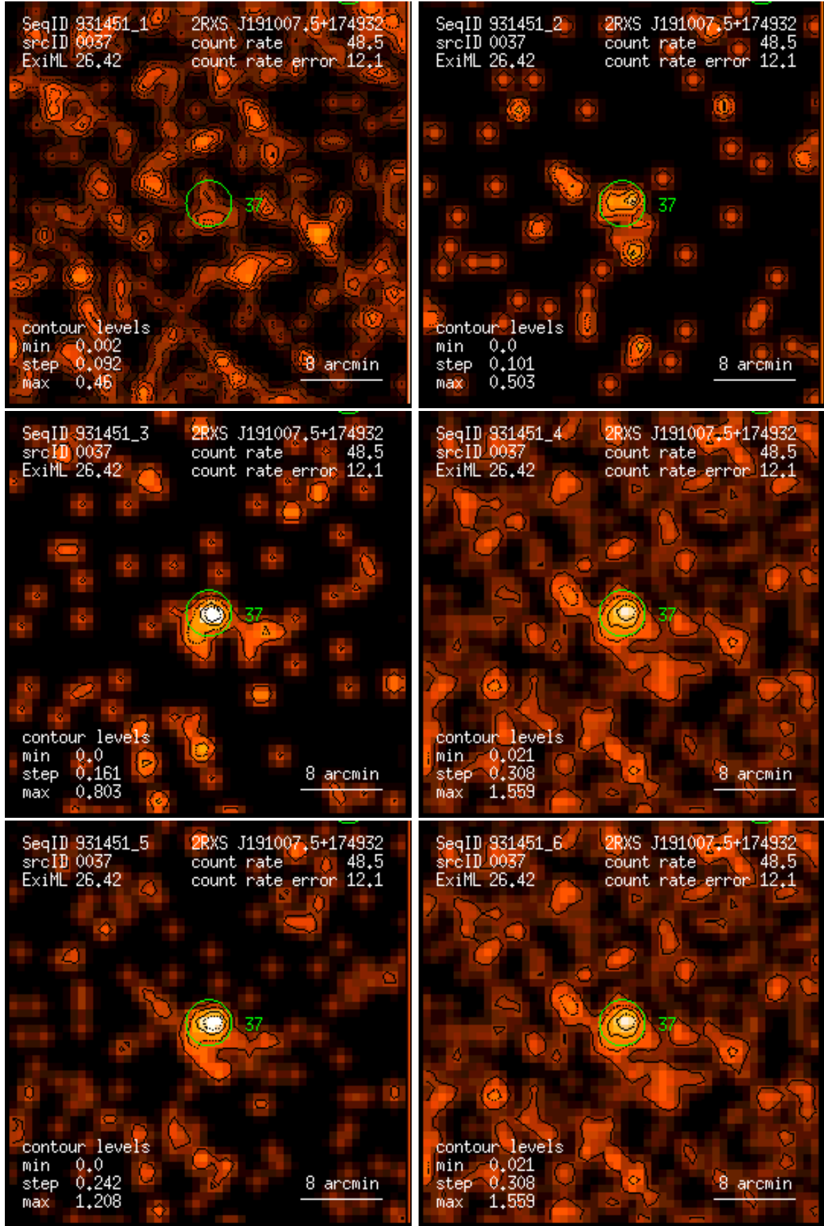
Figure 37: RASS 931451: detection 0037: band rate images, Gaussian filter: (1) PSPC channels 11 – 41, (2) 52 – 90, (3) 91 – 201, (4) 11 – 235, (5) 52 – 201, (6) 11 – 201. Broad band rates in counts/ks. Band rate contour levels in counts/ks/arcmin 2 .
