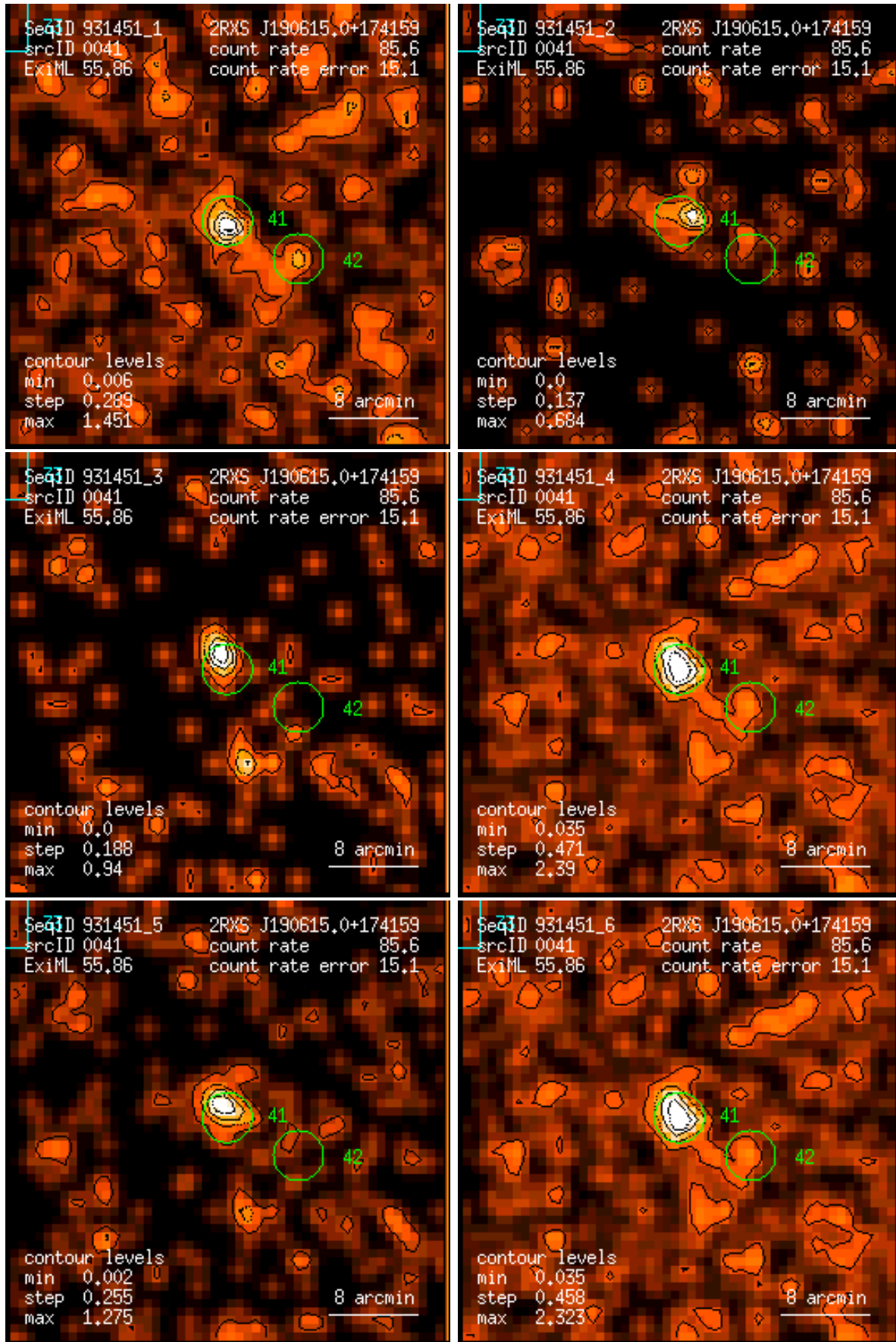
Figure 41: RASS 931451: detection 0041: band rate images, Gaussian filter: (1) PSPC channels 11 – 41, (2) 52 – 90, (3) 91 – 201, (4) 11 – 235, (5) 52 – 201, (6) 11 – 201. Broad band rates in counts/ks. Band rate contour levels in counts/ks/arcmin 2 .
