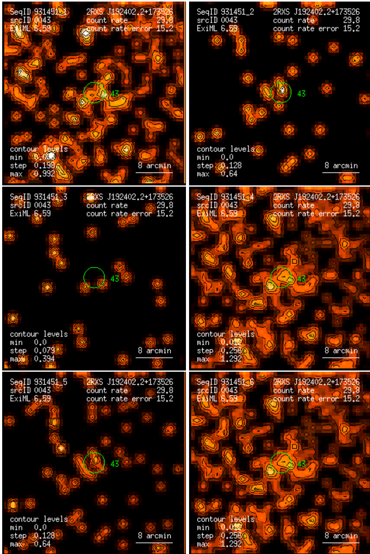
Figure 43: RASS 931451: detection 0043: band rate images, Gaussian filter: (1) PSPC channels 11 – 41, (2) 52 – 90, (3) 91 – 201, (4) 11 – 235, (5) 52 – 201, (6) 11 – 201. Broad band rates in counts/ks. Band rate contour levels in counts/ks/arcmin 2 .
