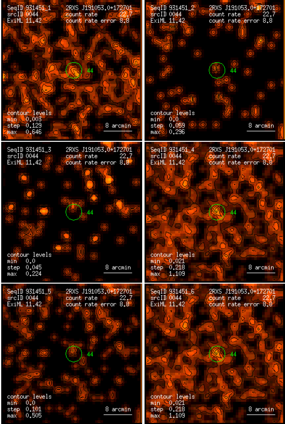
Figure 44: RASS 931451: detection 0044: band rate images, Gaussian filter: (1) PSPC channels 11 – 41, (2) 52 – 90, (3) 91 – 201, (4) 11 – 235, (5) 52 – 201, (6) 11 – 201. Broad band rates in counts/ks. Band rate contour levels in counts/ks/arcmin 2 .
