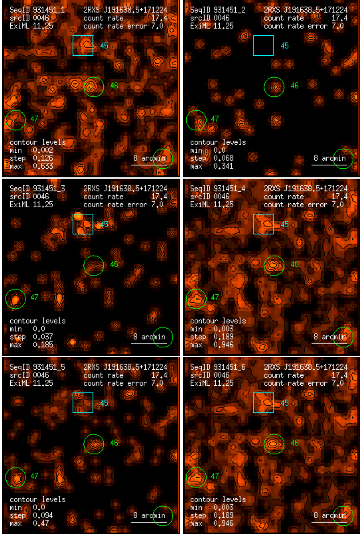
Figure 46: RASS 931451: detection 0046: band rate images, Gaussian filter: (1) PSPC channels 11 – 41, (2) 52 – 90, (3) 91 – 201, (4) 11 – 235, (5) 52 – 201, (6) 11 – 201. Broad band rates in counts/ks. Band rate contour levels in counts/ks/arcmin 2 .
