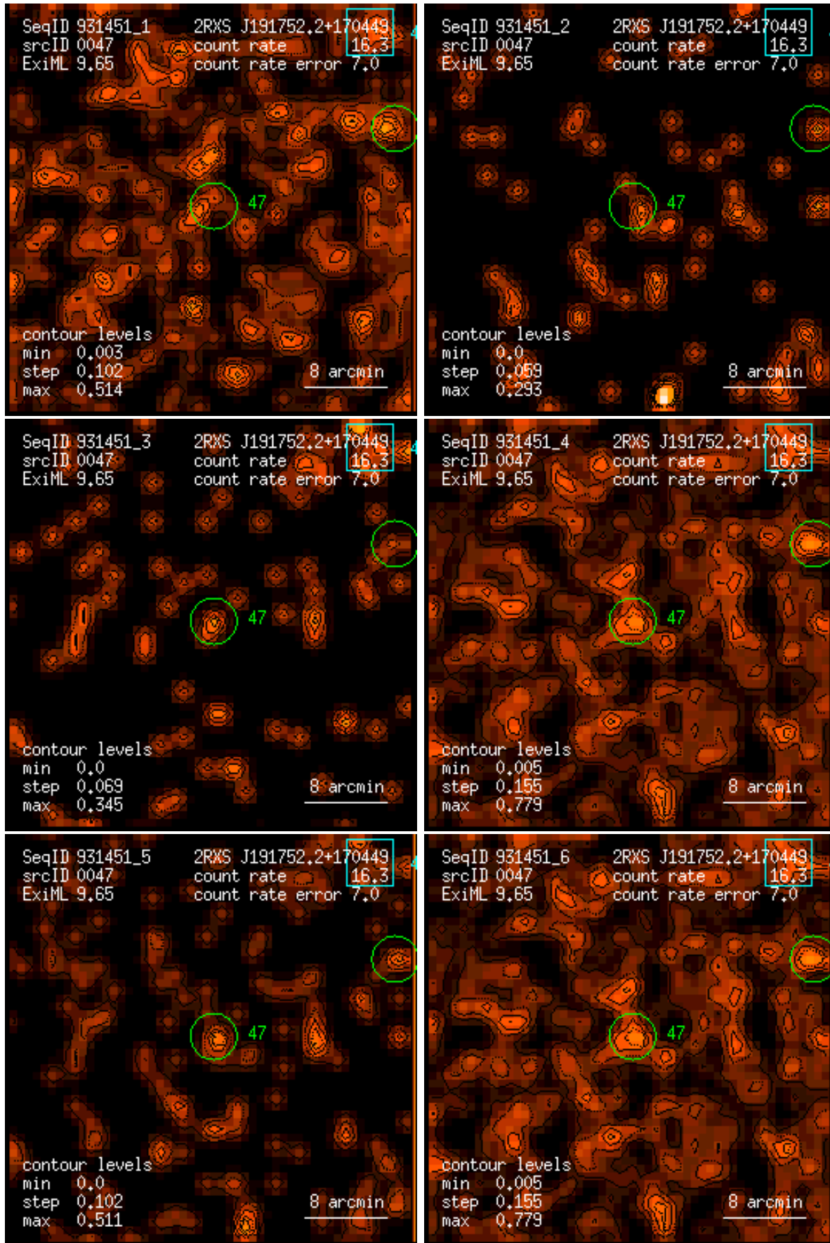
Figure 47: RASS 931451: detection 0047: band rate images, Gaussian filter: (1) PSPC channels 11 – 41, (2) 52 – 90, (3) 91 – 201, (4) 11 – 235, (5) 52 – 201, (6) 11 – 201. Broad band rates in counts/ks. Band rate contour levels in counts/ks/arcmin 2 .
