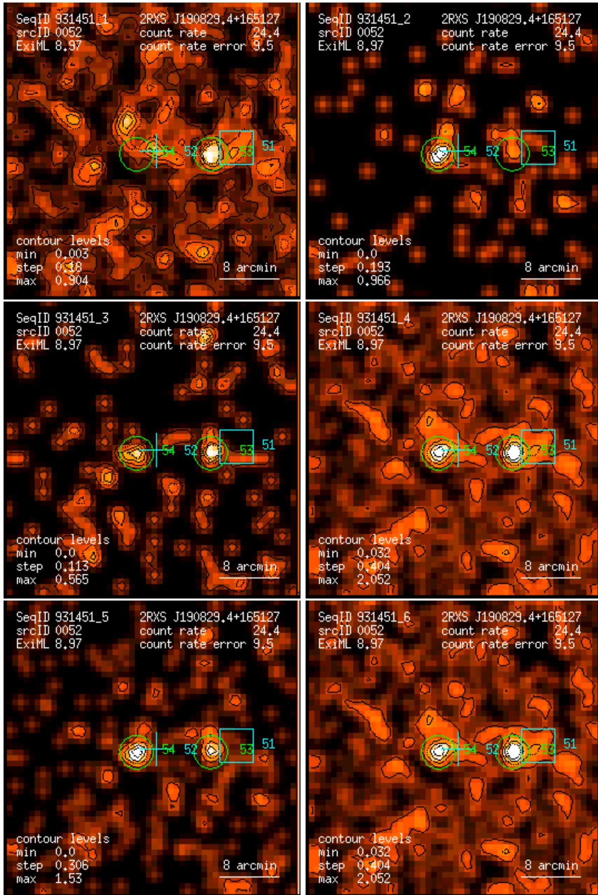
Figure 52: RASS 931451: detection 0052: band rate images, Gaussian filter: (1) PSPC channels 11 – 41, (2) 52 – 90, (3) 91 – 201, (4) 11 – 235, (5) 52 – 201, (6) 11 – 201. Broad band rates in counts/ks. Band rate contour levels in counts/ks/arcmin 2 .
