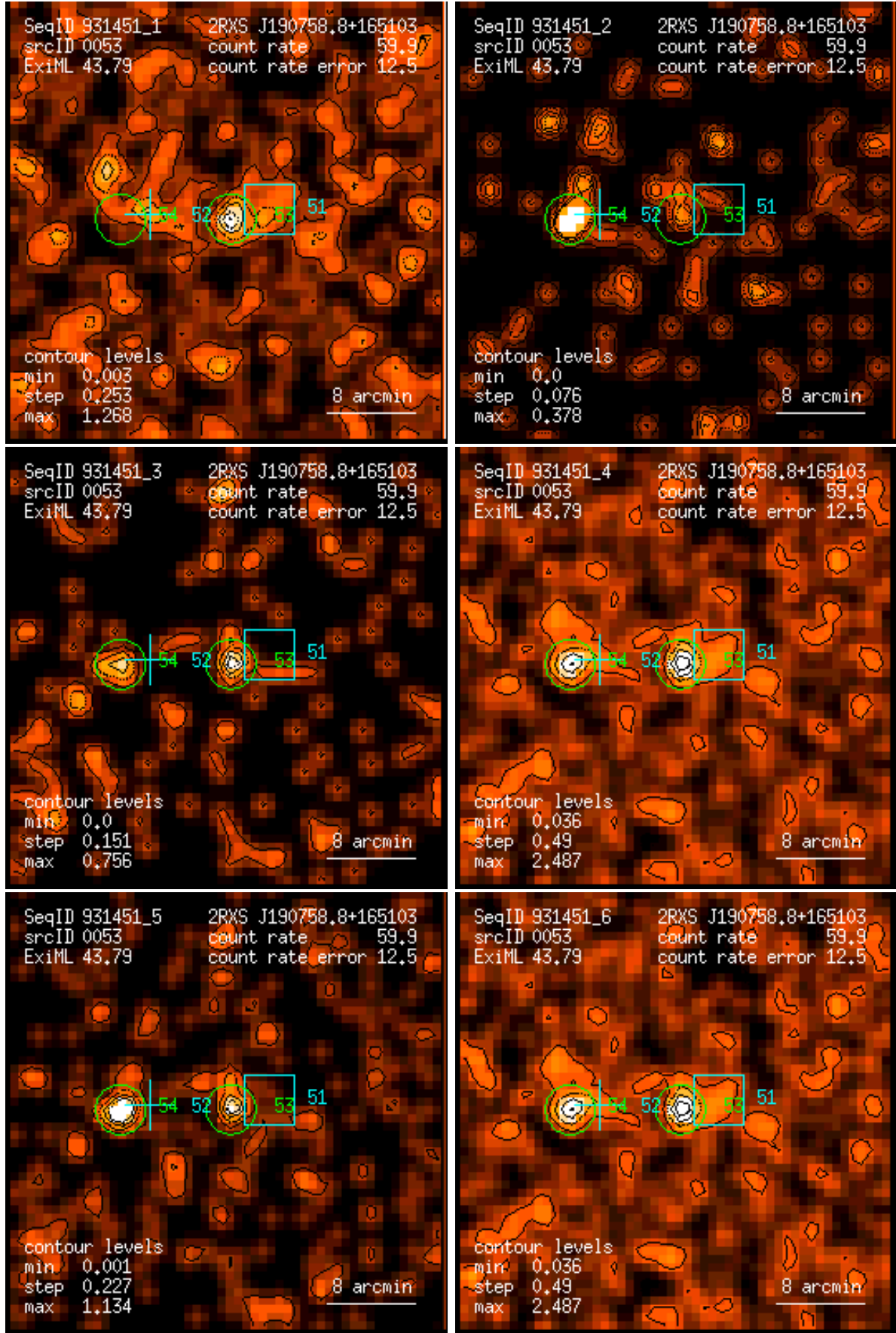
Figure 53: RASS 931451: detection 0053: band rate images, Gaussian filter: (1) PSPC channels 11 – 41, (2) 52 – 90, (3) 91 – 201, (4) 11 – 235, (5) 52 – 201, (6) 11 – 201. Broad band rates in counts/ks. Band rate contour levels in counts/ks/arcmin 2 .
