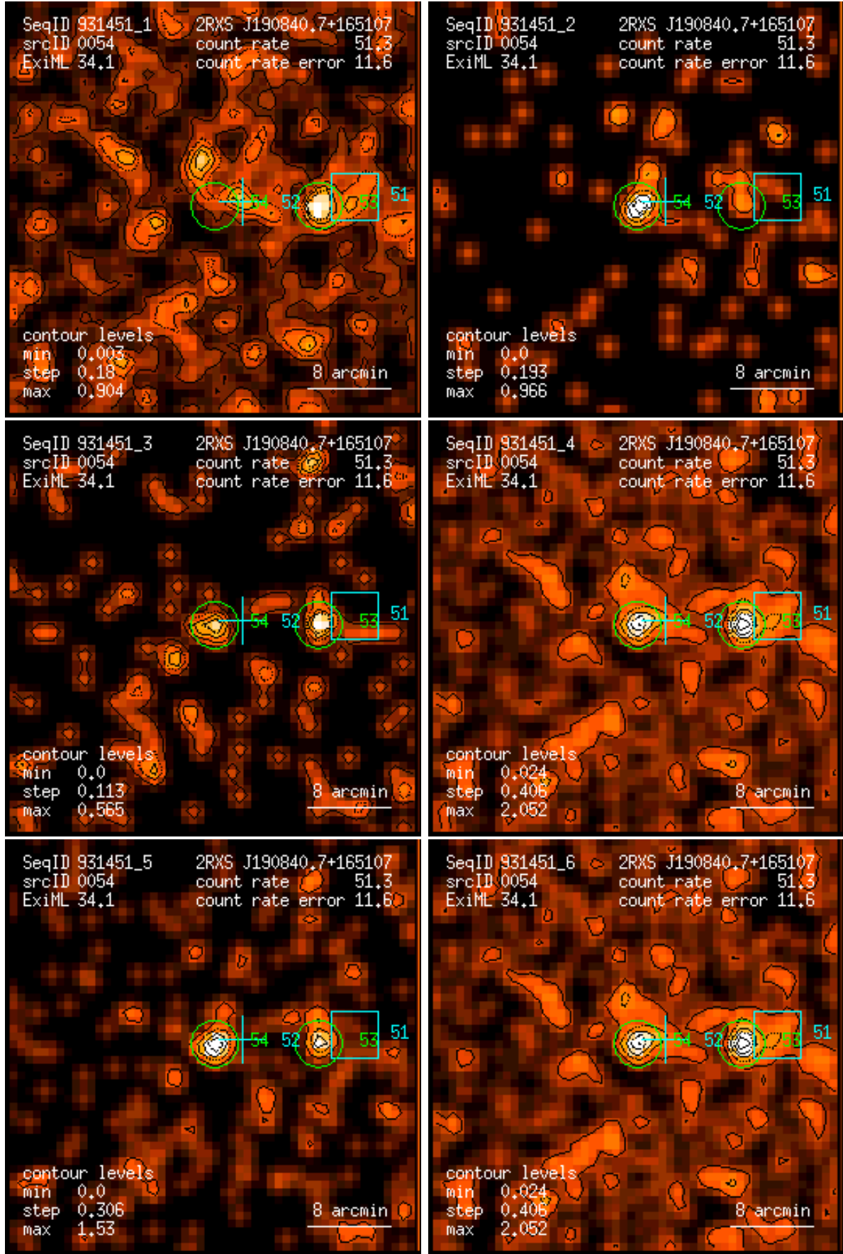
Figure 54: RASS 931451: detection 0054: band rate images, Gaussian filter: (1) PSPC channels 11 – 41, (2) 52 – 90, (3) 91 – 201, (4) 11 – 235, (5) 52 – 201, (6) 11 – 201. Broad band rates in counts/ks. Band rate contour levels in counts/ks/arcmin 2 .
