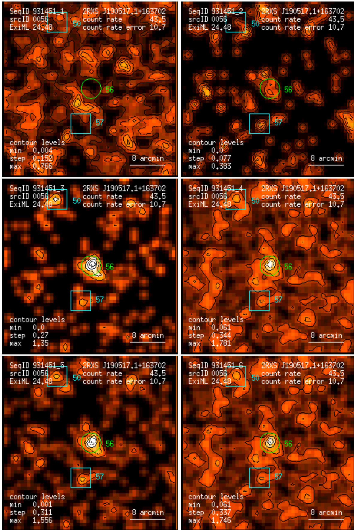
Figure 56: RASS 931451: detection 0056: band rate images, Gaussian filter: (1) PSPC channels 11 – 41, (2) 52 – 90, (3) 91 – 201, (4) 11 – 235, (5) 52 – 201, (6) 11 – 201. Broad band rates in counts/ks. Band rate contour levels in counts/ks/arcmin 2 .
