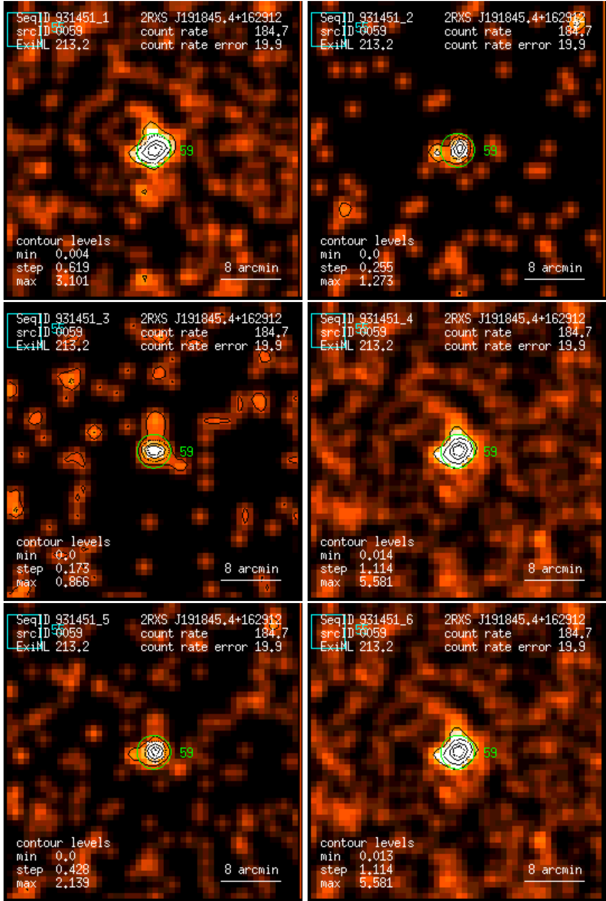
Figure 59: RASS 931451: detection 0059: band rate images, Gaussian filter: (1) PSPC channels 11 – 41, (2) 52 – 90, (3) 91 – 201, (4) 11 – 235, (5) 52 – 201, (6) 11 – 201. Broad band rates in counts/ks. Band rate contour levels in counts/ks/arcmin 2 .
