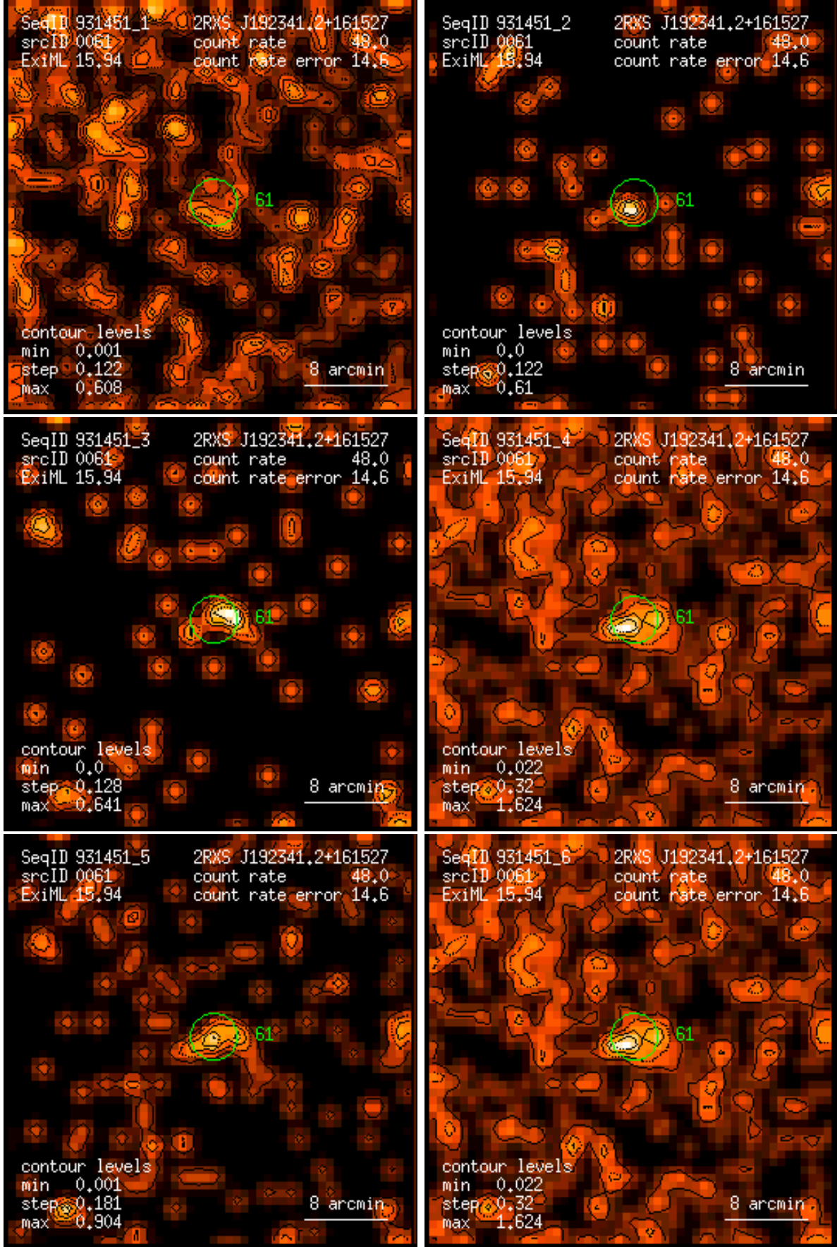
Figure 61: RASS 931451: detection 0061: band rate images, Gaussian filter: (1) PSPC channels 11 – 41, (2) 52 – 90, (3) 91 – 201, (4) 11 – 235, (5) 52 – 201, (6) 11 – 201. Broad band rates in counts/ks. Band rate contour levels in counts/ks/arcmin 2 .
