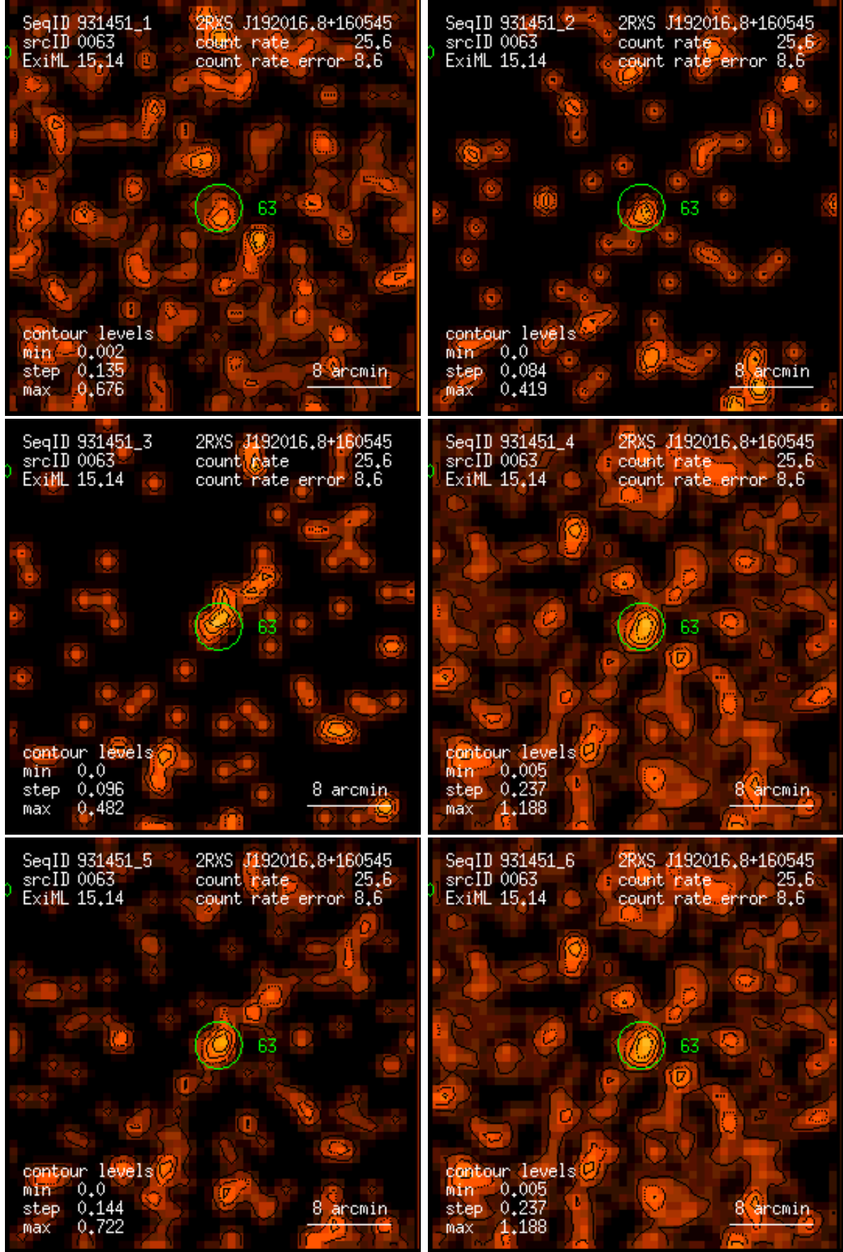
Figure 63: RASS 931451: detection 0063: band rate images, Gaussian filter: (1) PSPC channels 11 – 41, (2) 52 – 90, (3) 91 – 201, (4) 11 – 235, (5) 52 – 201, (6) 11 – 201. Broad band rates in counts/ks. Band rate contour levels in counts/ks/arcmin 2 .
