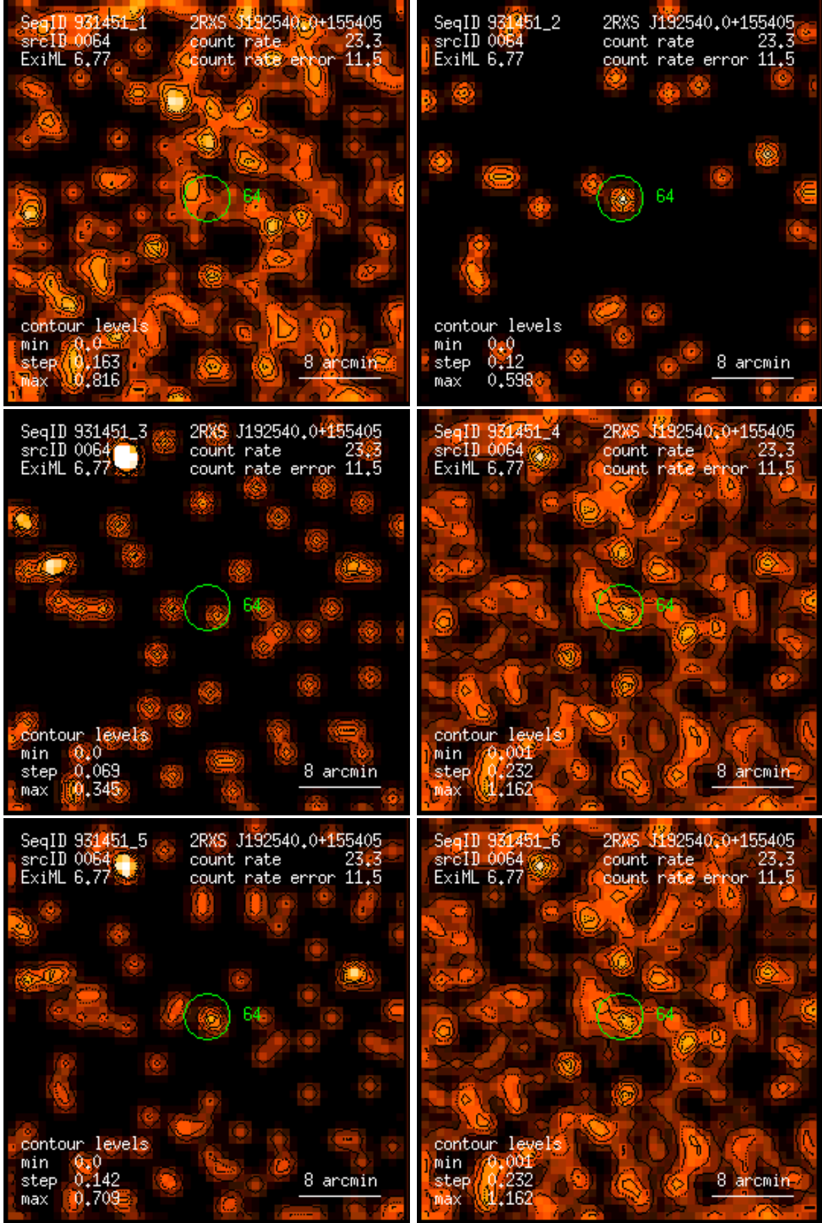
Figure 64: RASS 931451: detection 0064: band rate images, Gaussian filter: (1) PSPC channels 11 – 41, (2) 52 – 90, (3) 91 – 201, (4) 11 – 235, (5) 52 – 201, (6) 11 – 201. Broad band rates in counts/ks. Band rate contour levels in counts/ks/arcmin 2 .
