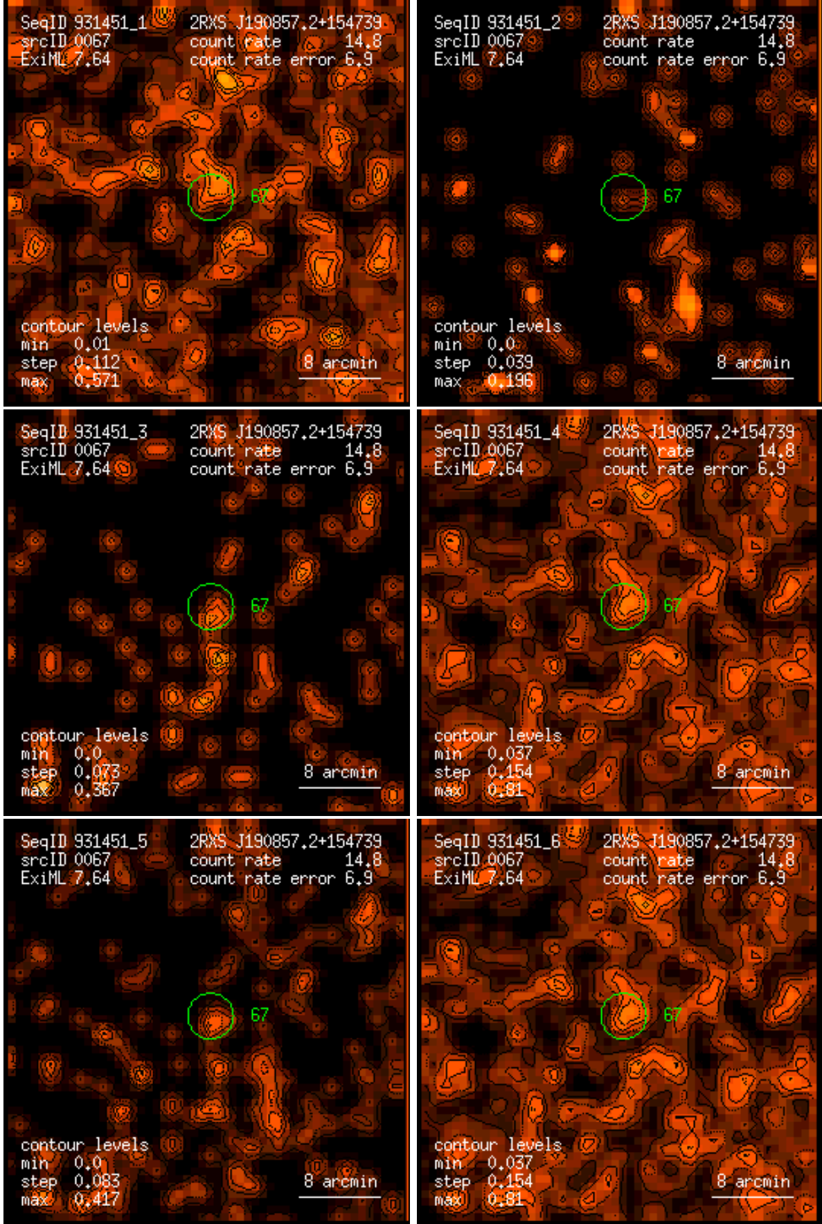
Figure 67: RASS 931451: detection 0067: band rate images, Gaussian filter: (1) PSPC channels 11 – 41, (2) 52 – 90, (3) 91 – 201, (4) 11 – 235, (5) 52 – 201, (6) 11 – 201. Broad band rates in counts/ks. Band rate contour levels in counts/ks/arcmin 2 .
