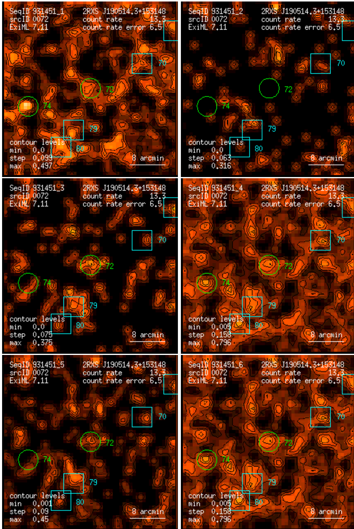
Figure 72: RASS 931451: detection 0072: band rate images, Gaussian filter: (1) PSPC channels 11 – 41, (2) 52 – 90, (3) 91 – 201, (4) 11 – 235, (5) 52 – 201, (6) 11 – 201. Broad band rates in counts/ks. Band rate contour levels in counts/ks/arcmin 2 .
