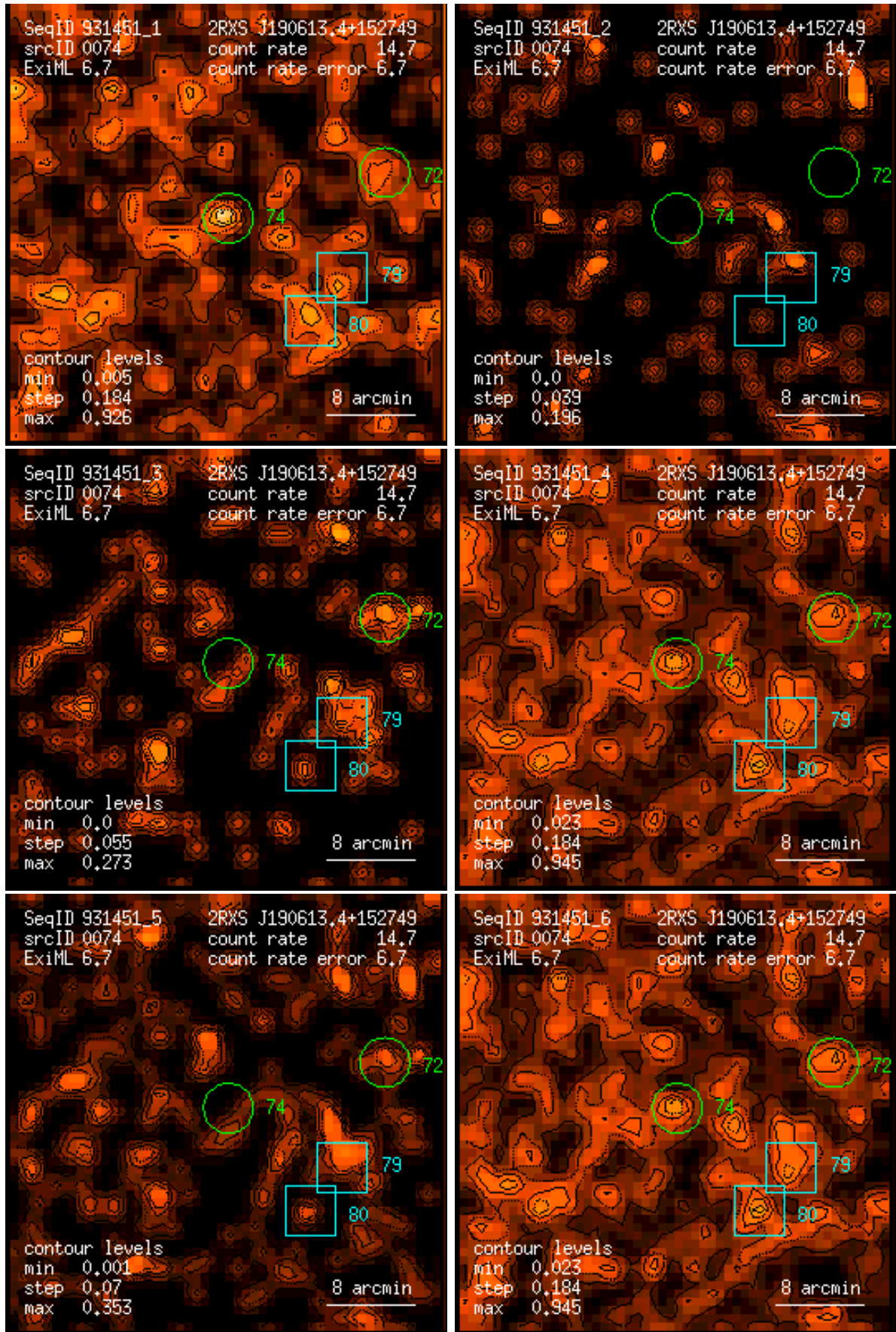
Figure 74: RASS 931451: detection 0074: band rate images, Gaussian filter: (1) PSPC channels 11 – 41, (2) 52 – 90, (3) 91 – 201, (4) 11 – 235, (5) 52 – 201, (6) 11 – 201. Broad band rates in counts/ks. Band rate contour levels in counts/ks/arcmin 2 .
