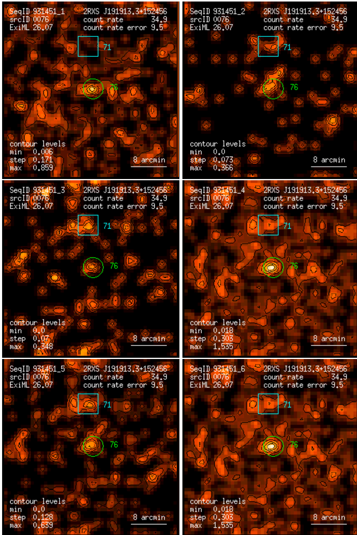
Figure 76: RASS 931451: detection 0076: band rate images, Gaussian filter: (1) PSPC channels 11 – 41, (2) 52 – 90, (3) 91 – 201, (4) 11 – 235, (5) 52 – 201, (6) 11 – 201. Broad band rates in counts/ks. Band rate contour levels in counts/ks/arcmin 2 .
