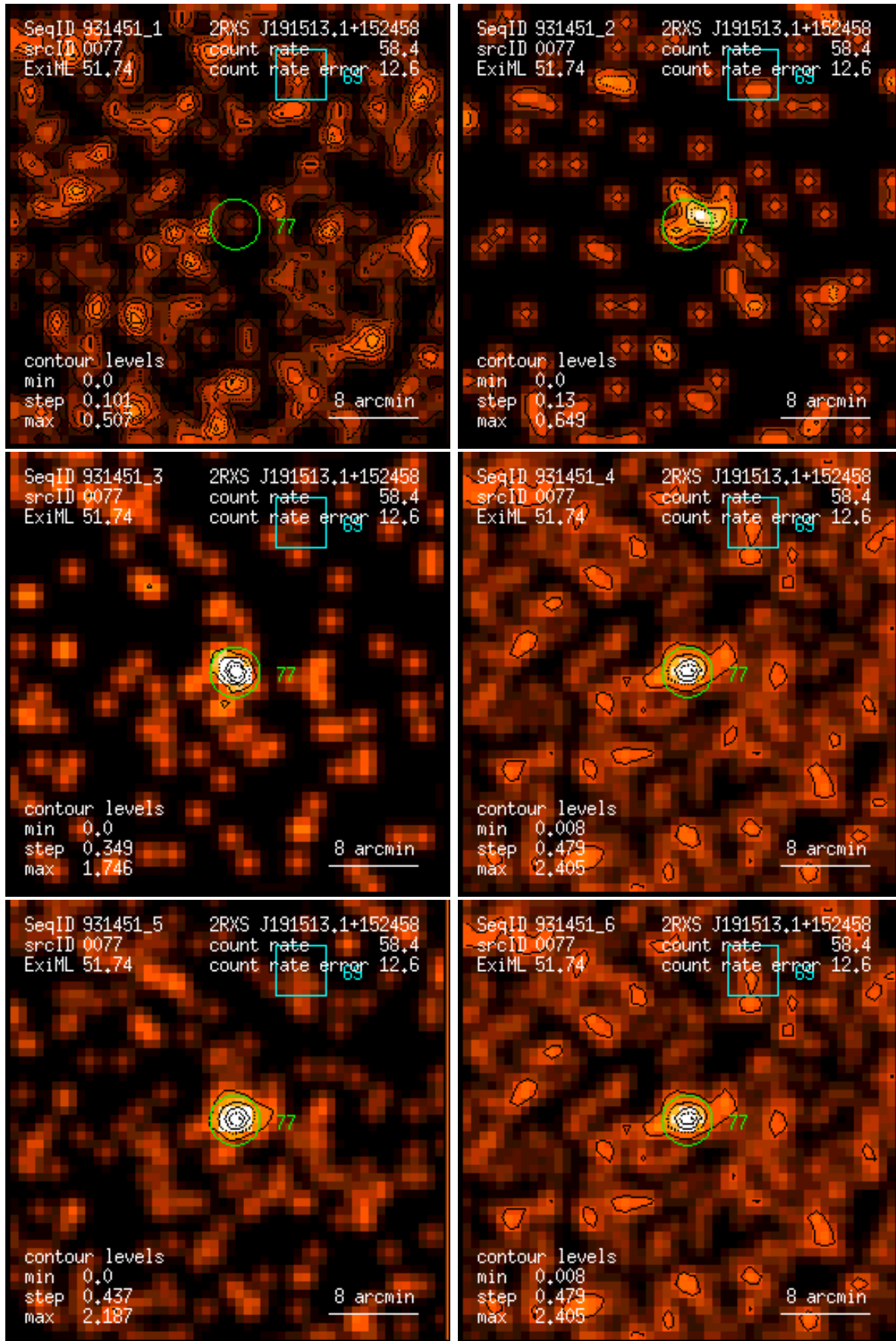
Figure 77: RASS 931451: detection 0077: band rate images, Gaussian filter: (1) PSPC channels 11 – 41, (2) 52 – 90, (3) 91 – 201, (4) 11 – 235, (5) 52 – 201, (6) 11 – 201. Broad band rates in counts/ks. Band rate contour levels in counts/ks/arcmin 2 .
