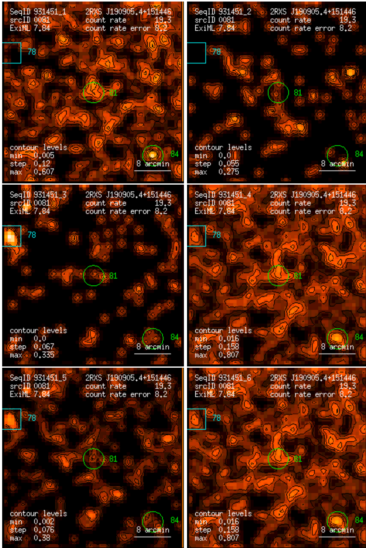
Figure 81: RASS 931451: detection 0081: band rate images, Gaussian filter: (1) PSPC channels 11 – 41, (2) 52 – 90, (3) 91 – 201, (4) 11 – 235, (5) 52 – 201, (6) 11 – 201. Broad band rates in counts/ks. Band rate contour levels in counts/ks/arcmin 2 .
