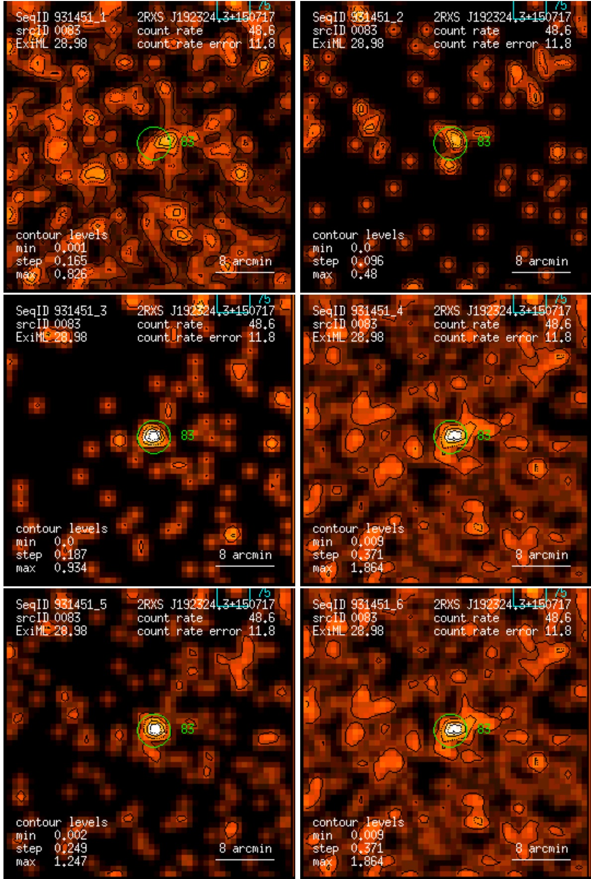
Figure 83: RASS 931451: detection 0083: band rate images, Gaussian filter: (1) PSPC channels 11 – 41, (2) 52 – 90, (3) 91 – 201, (4) 11 – 235, (5) 52 – 201, (6) 11 – 201. Broad band rates in counts/ks. Band rate contour levels in counts/ks/arcmin 2 .
