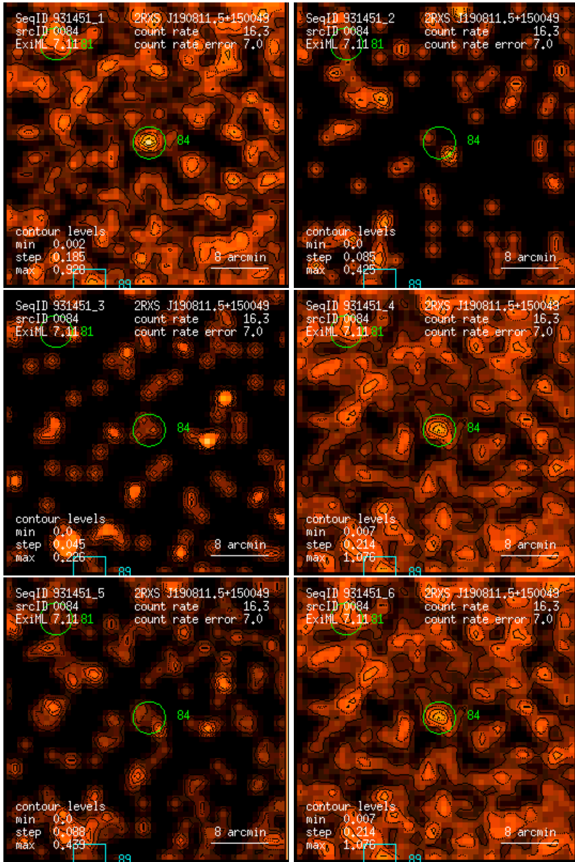
Figure 84: RASS 931451: detection 0084: band rate images, Gaussian filter: (1) PSPC channels 11 – 41, (2) 52 – 90, (3) 91 – 201, (4) 11 – 235, (5) 52 – 201, (6) 11 – 201. Broad band rates in counts/ks. Band rate contour levels in counts/ks/arcmin 2 .
