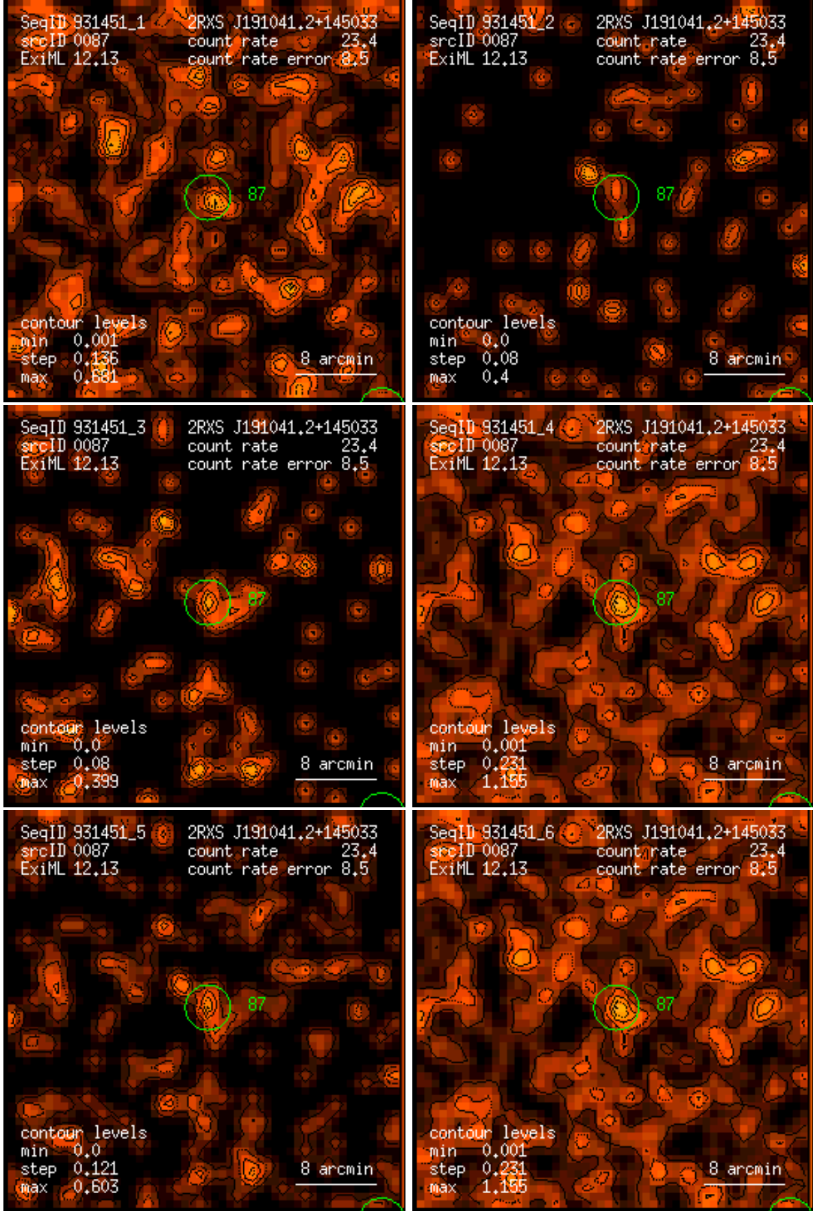
Figure 87: RASS 931451: detection 0087: band rate images, Gaussian filter: (1) PSPC channels 11 – 41, (2) 52 – 90, (3) 91 – 201, (4) 11 – 235, (5) 52 – 201, (6) 11 – 201. Broad band rates in counts/ks. Band rate contour levels in counts/ks/arcmin 2 .
