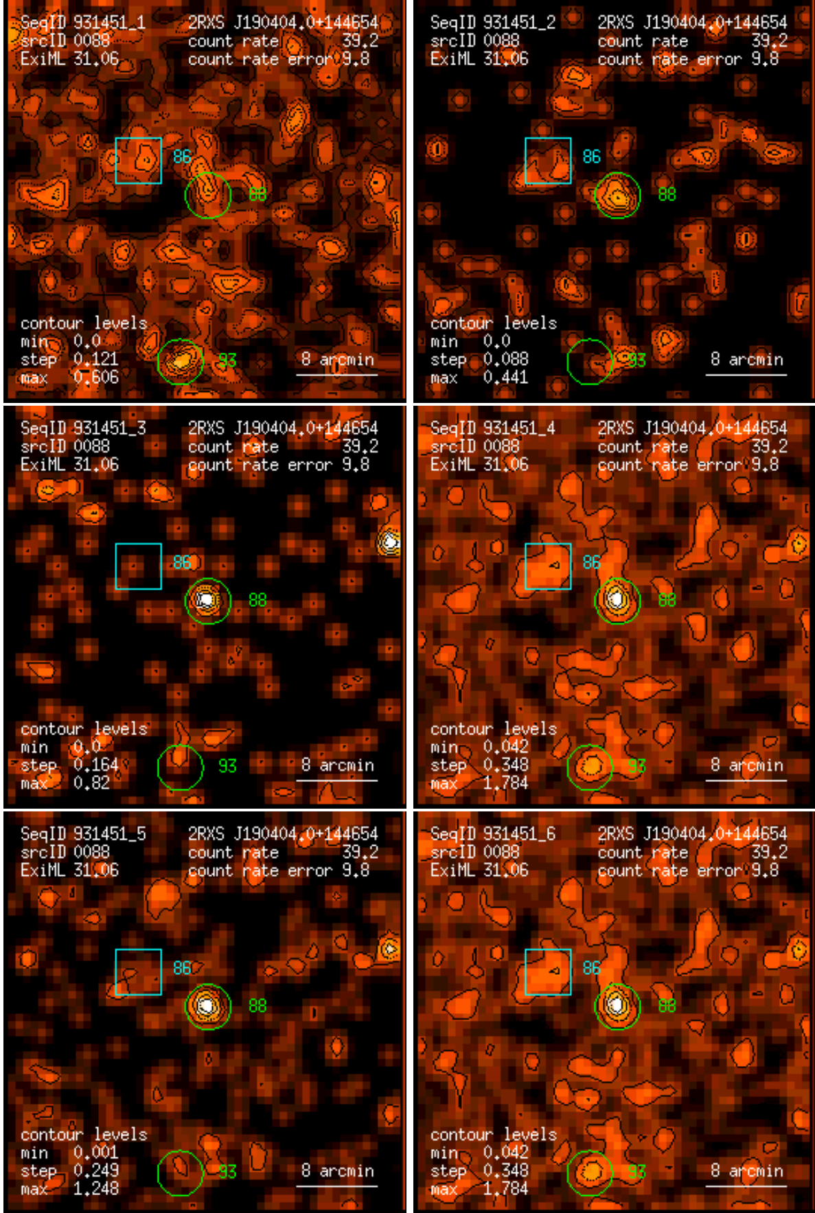
Figure 88: RASS 931451: detection 0088: band rate images, Gaussian filter: (1) PSPC channels 11 – 41, (2) 52 – 90, (3) 91 – 201, (4) 11 – 235, (5) 52 – 201, (6) 11 – 201. Broad band rates in counts/ks. Band rate contour levels in counts/ks/arcmin 2 .
