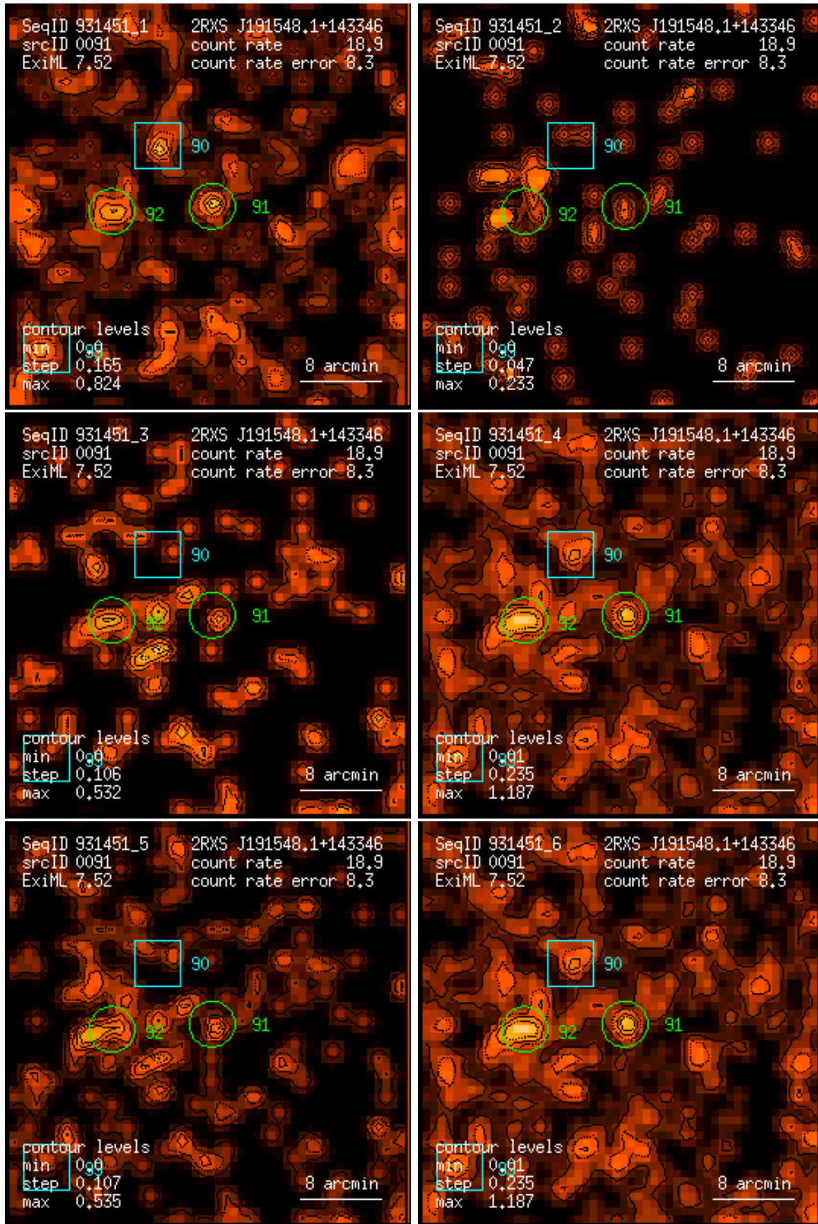
Figure 91: RASS 931451: detection 0091: band rate images, Gaussian filter: (1) PSPC channels 11 – 41, (2) 52 – 90, (3) 91 – 201, (4) 11 – 235, (5) 52 – 201, (6) 11 – 201. Broad band rates in counts/ks. Band rate contour levels in counts/ks/arcmin 2 .
