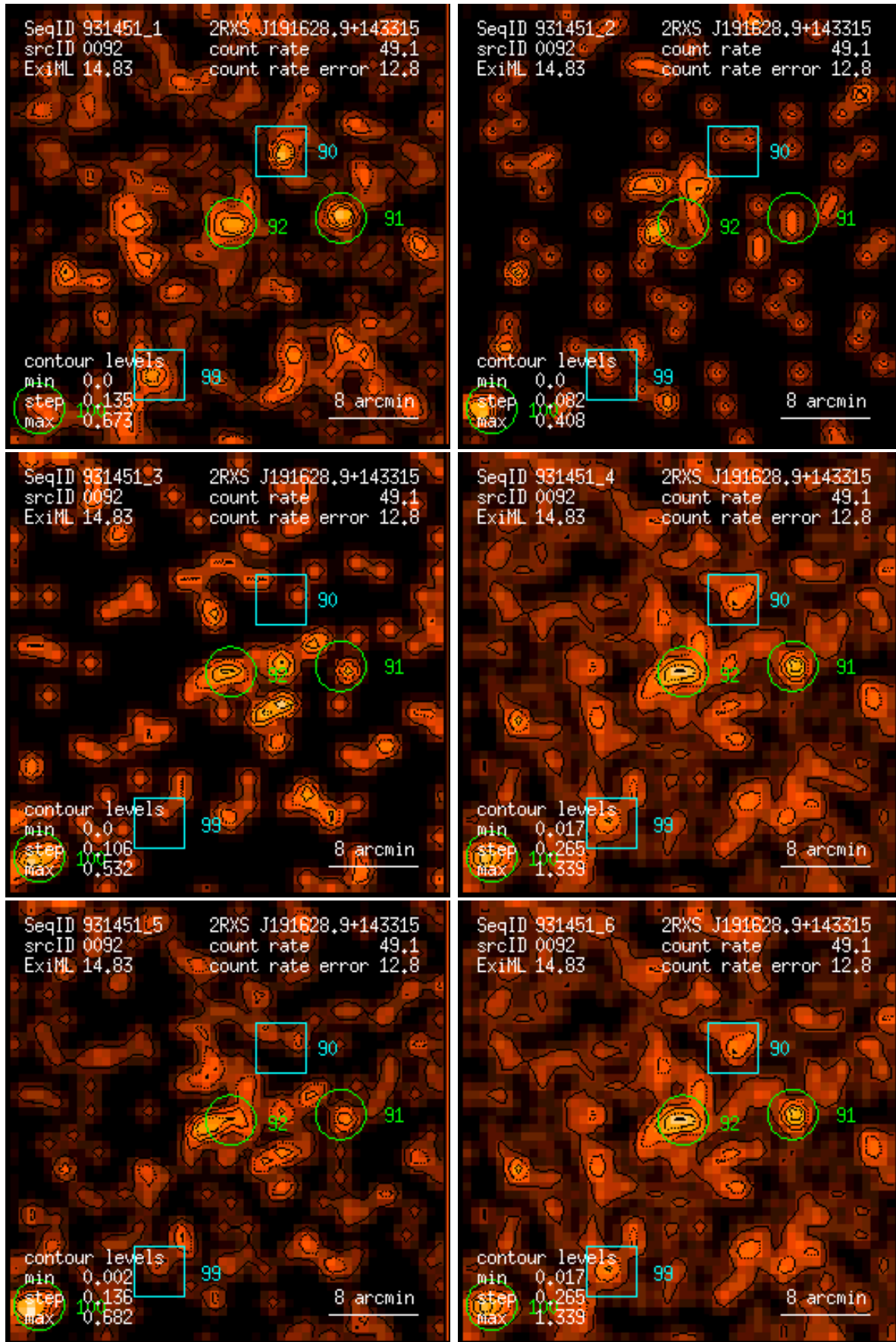
Figure 92: RASS 931451: detection 0092: band rate images, Gaussian filter: (1) PSPC channels 11 – 41, (2) 52 – 90, (3) 91 – 201, (4) 11 – 235, (5) 52 – 201, (6) 11 – 201. Broad band rates in counts/ks. Band rate contour levels in counts/ks/arcmin 2 .
