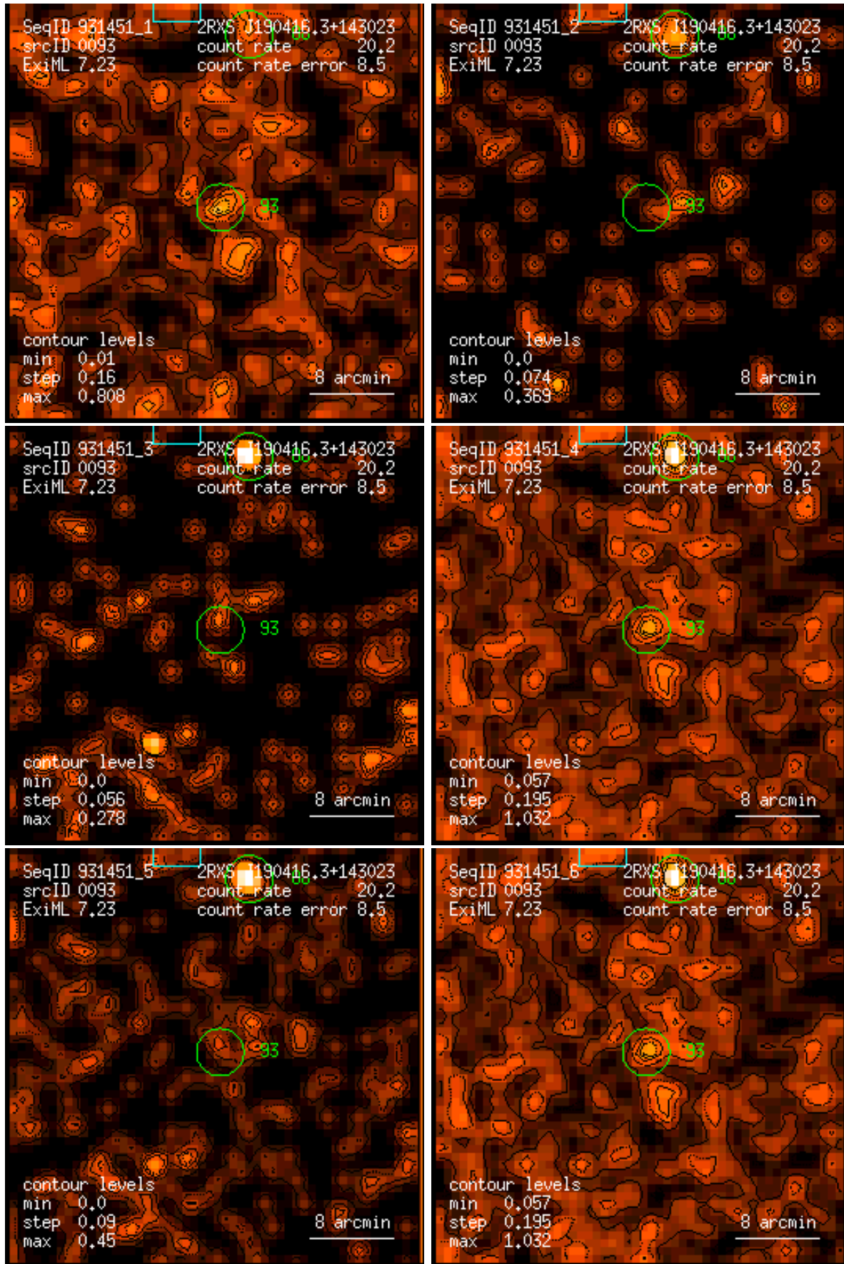
Figure 93: RASS 931451: detection 0093: band rate images, Gaussian filter: (1) PSPC channels 11 – 41, (2) 52 – 90, (3) 91 – 201, (4) 11 – 235, (5) 52 – 201, (6) 11 – 201. Broad band rates in counts/ks. Band rate contour levels in counts/ks/arcmin 2 .
