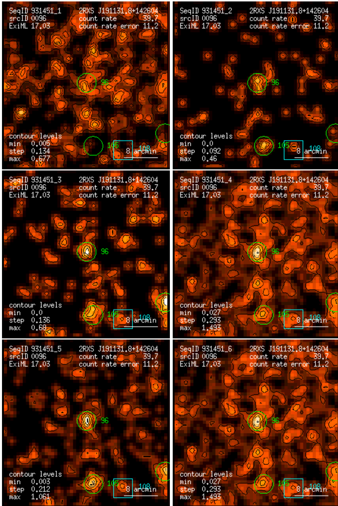
Figure 96: RASS 931451: detection 0096: band rate images, Gaussian filter: (1) PSPC channels 11 – 41, (2) 52 – 90, (3) 91 – 201, (4) 11 – 235, (5) 52 – 201, (6) 11 – 201. Broad band rates in counts/ks. Band rate contour levels in counts/ks/arcmin 2 .
