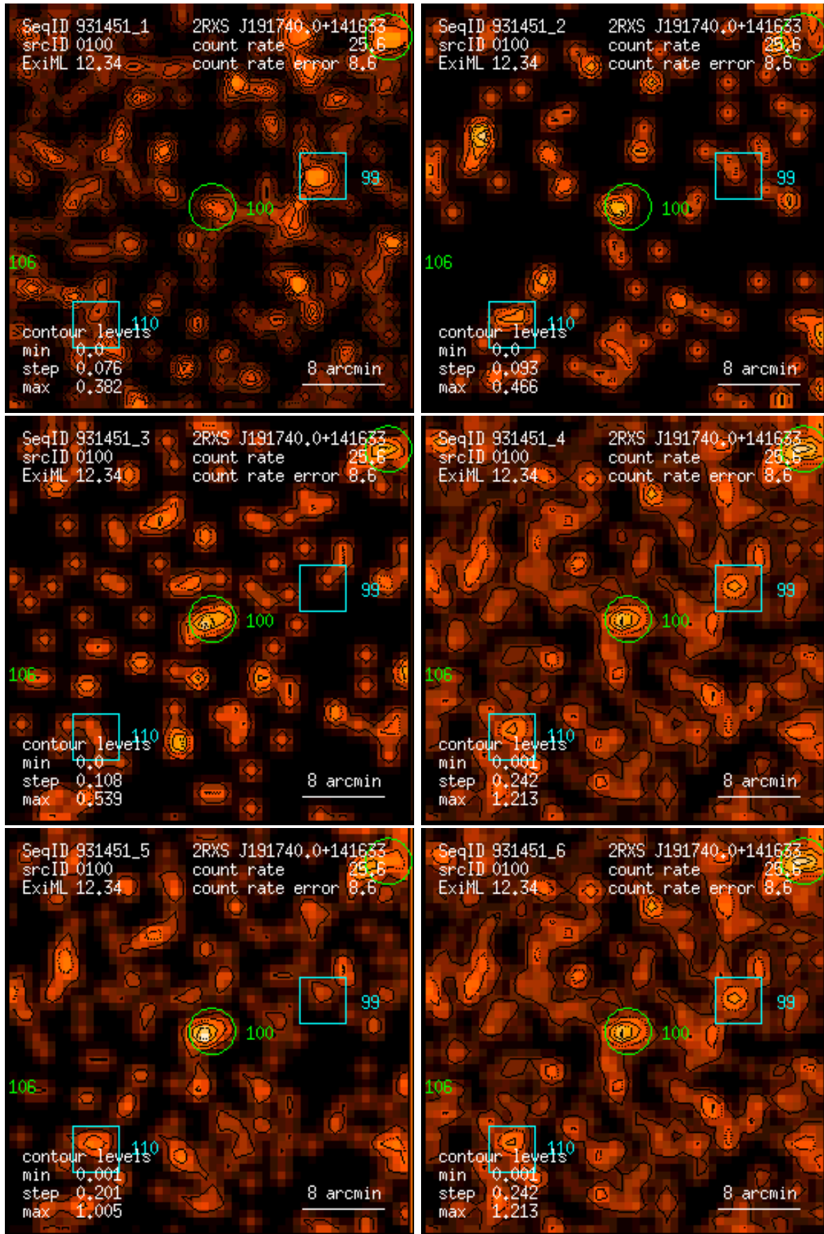
Figure 100: RASS 931451: detection 0100: band rate images, Gaussian filter: (1) PSPC channels 11 – 41, (2) 52 – 90, (3) 91 – 201, (4) 11 – 235, (5) 52 – 201, (6) 11 – 201. Broad band rates in counts/ks. Band rate contour levels in counts/ks/arcmin 2 .
