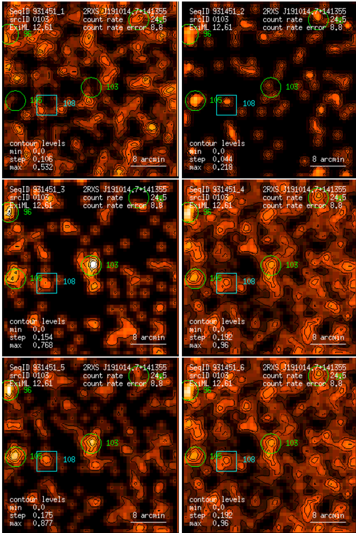
Figure 103: RASS 931451: detection 0103: band rate images, Gaussian filter: (1) PSPC channels 11 – 41, (2) 52 – 90, (3) 91 – 201, (4) 11 – 235, (5) 52 – 201, (6) 11 – 201. Broad band rates in counts/ks. Band rate contour levels in counts/ks/arcmin 2 .
