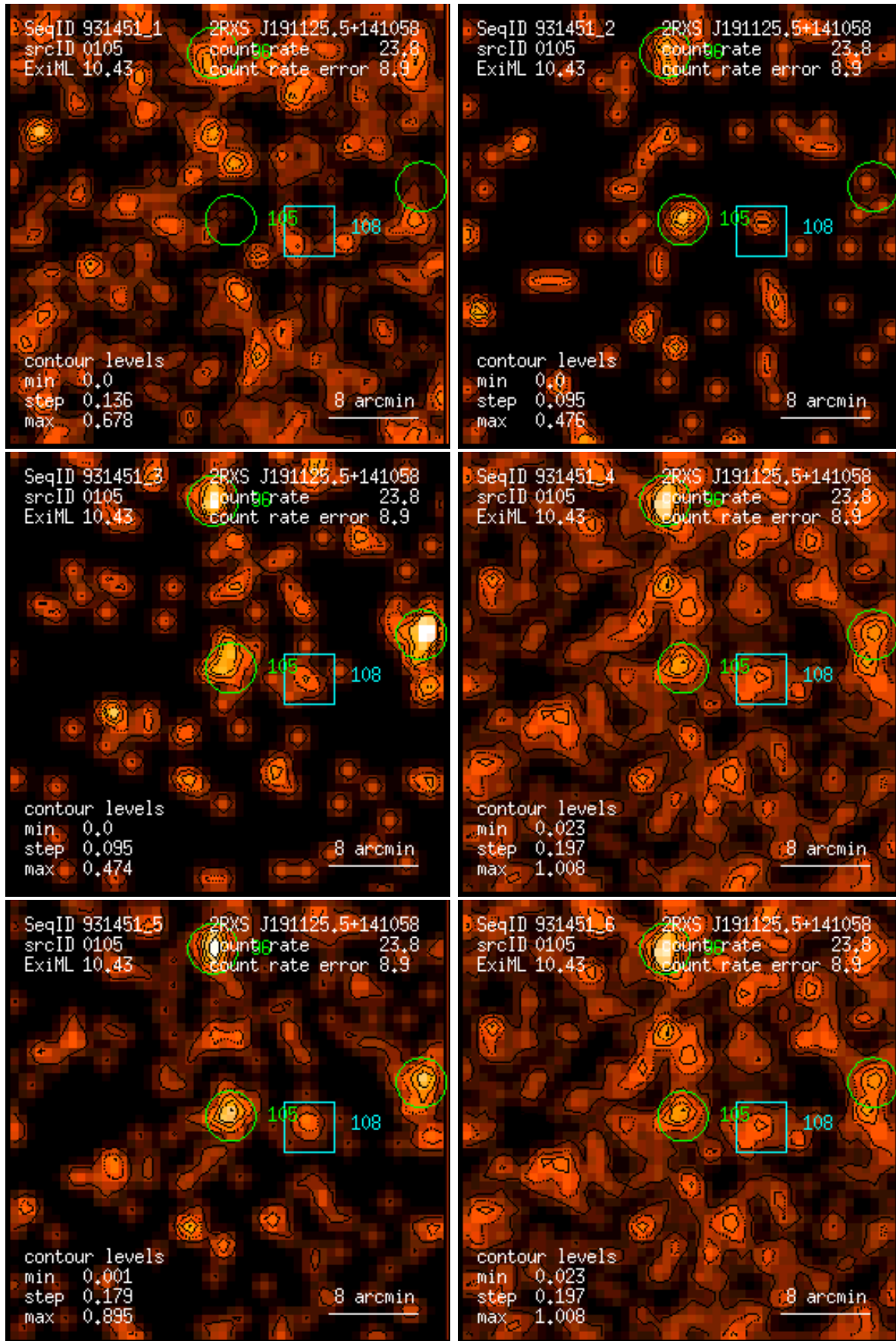
Figure 105: RASS 931451: detection 0105: band rate images, Gaussian filter: (1) PSPC channels 11 – 41, (2) 52 – 90, (3) 91 – 201, (4) 11 – 235, (5) 52 – 201, (6) 11 – 201. Broad band rates in counts/ks. Band rate contour levels in counts/ks/arcmin 2 .
