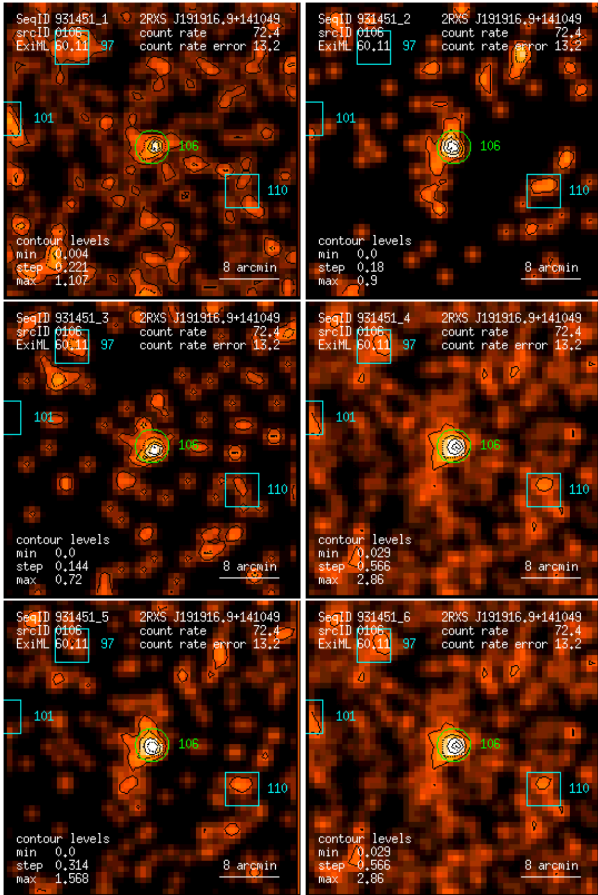
Figure 106: RASS 931451: detection 0106: band rate images, Gaussian filter: (1) PSPC channels 11 – 41, (2) 52 – 90, (3) 91 – 201, (4) 11 – 235, (5) 52 – 201, (6) 11 – 201. Broad band rates in counts/ks. Band rate contour levels in counts/ks/arcmin 2 .
