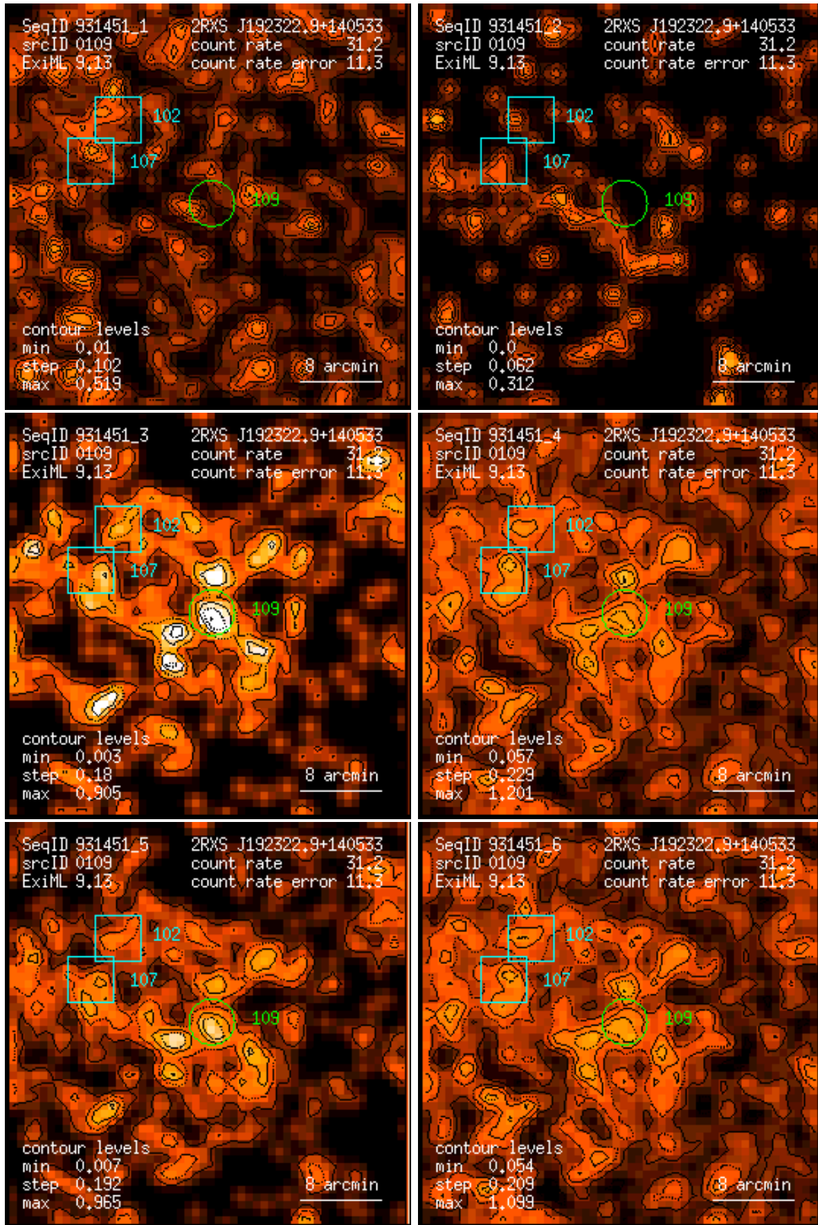
Figure 109: RASS 931451: detection 0109: band rate images, Gaussian filter: (1) PSPC channels 11 – 41, (2) 52 – 90, (3) 91 – 201, (4) 11 – 235, (5) 52 – 201, (6) 11 – 201. Broad band rates in counts/ks. Band rate contour levels in counts/ks/arcmin 2 .
